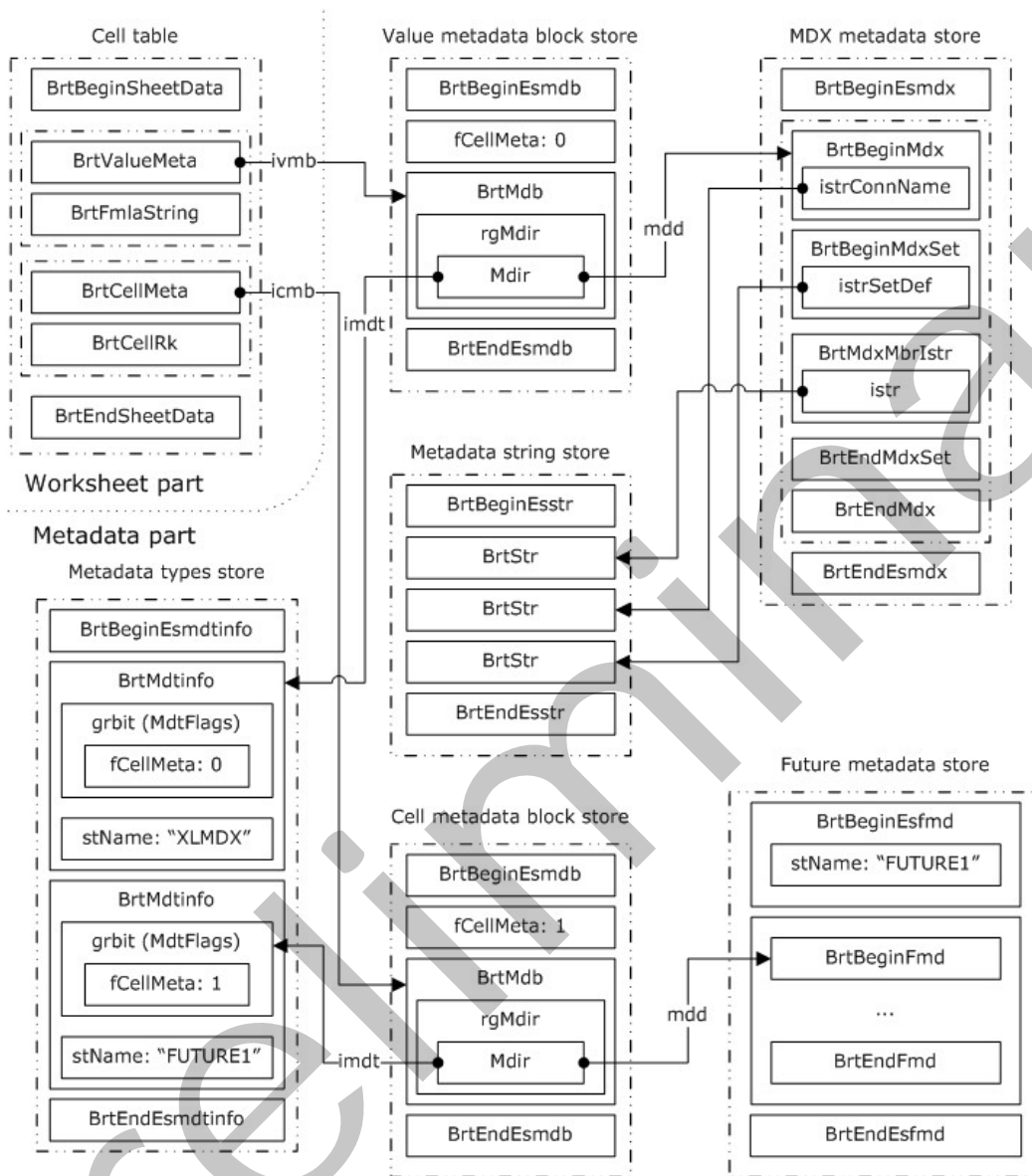
Figure 1: Metadata
