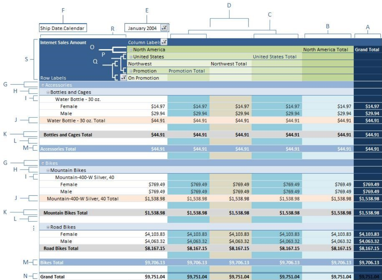
Figure 18: PivotTable-style diagram
