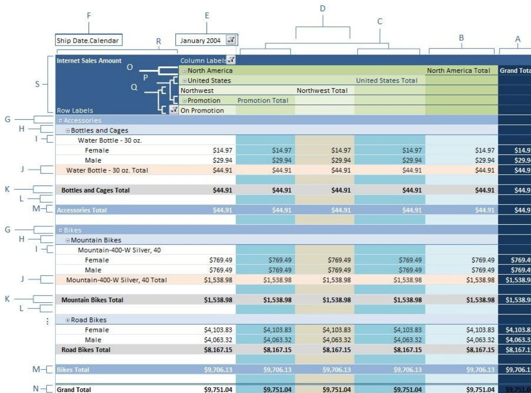
Figure 18: PivotTable-style diagram
