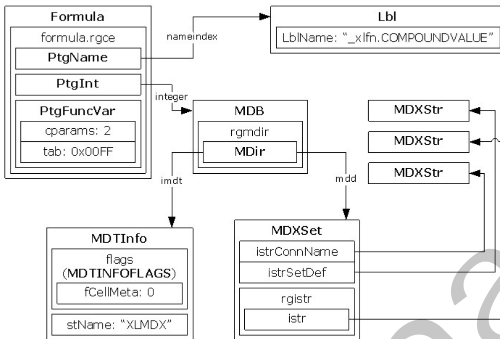
Figure 2: Metadata
