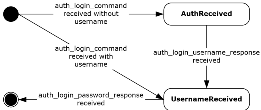
Figure 1: Server state machine diagram
