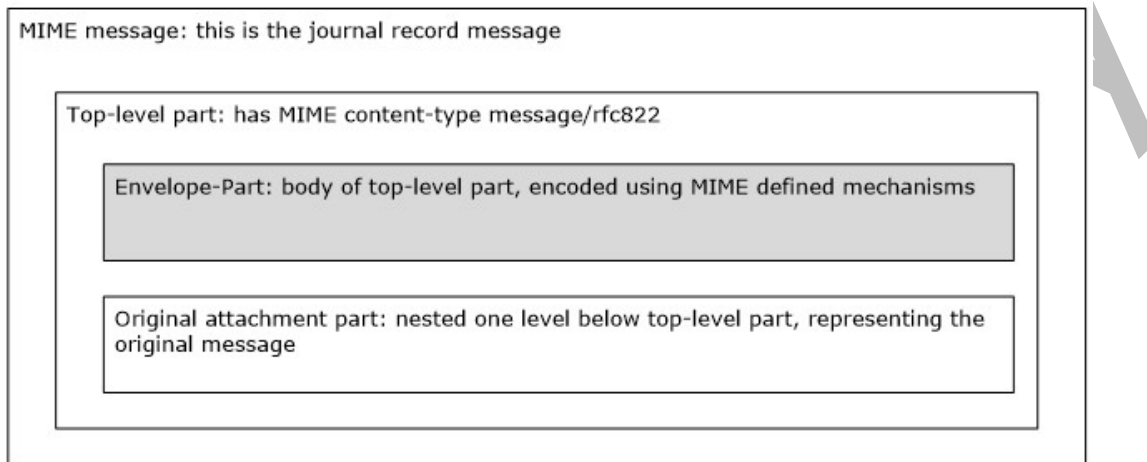
Figure 1: MIME structure of a journal record message
