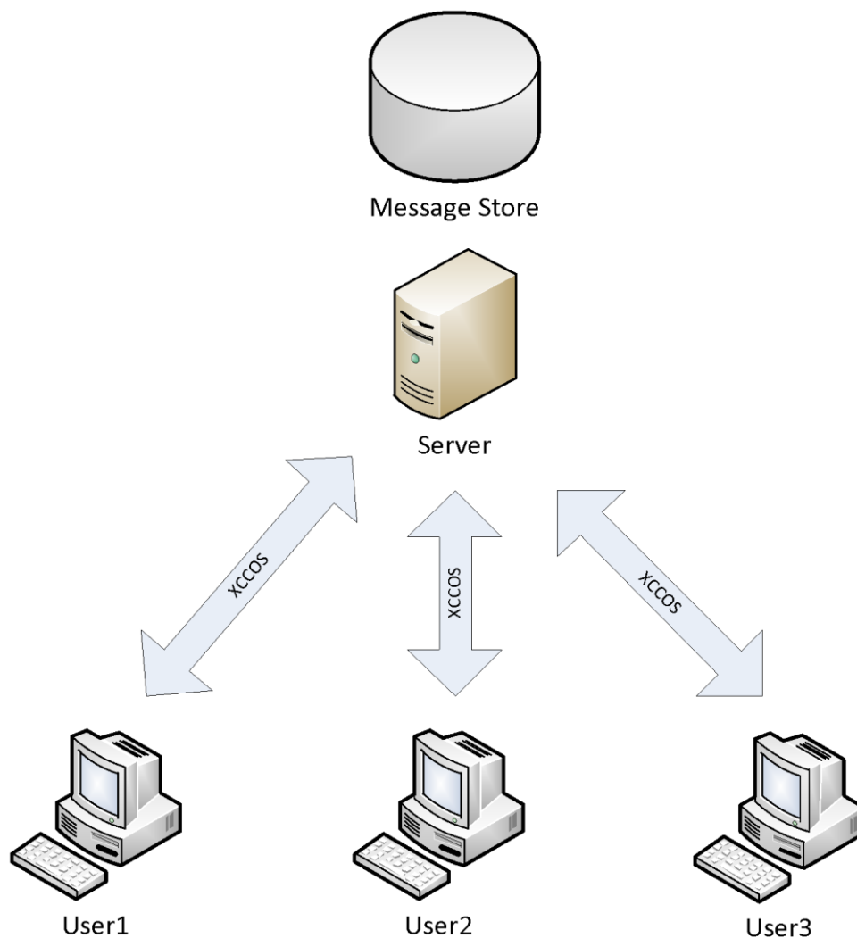
Figure 1: Sample implementation
