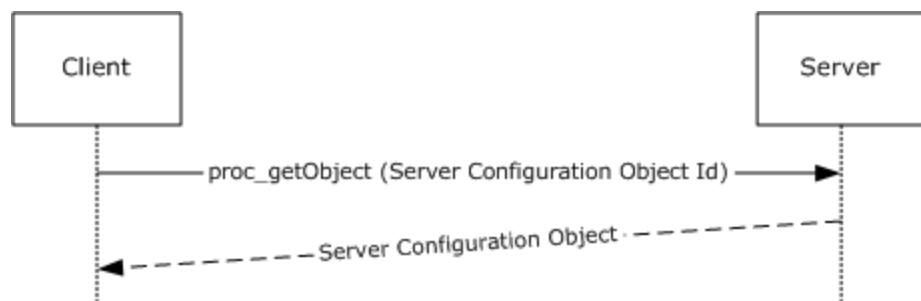
Figure 15: Server Address
