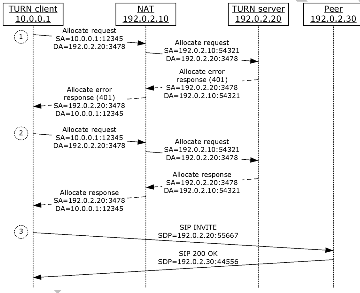
Figure 3: Example of TURN message flow
