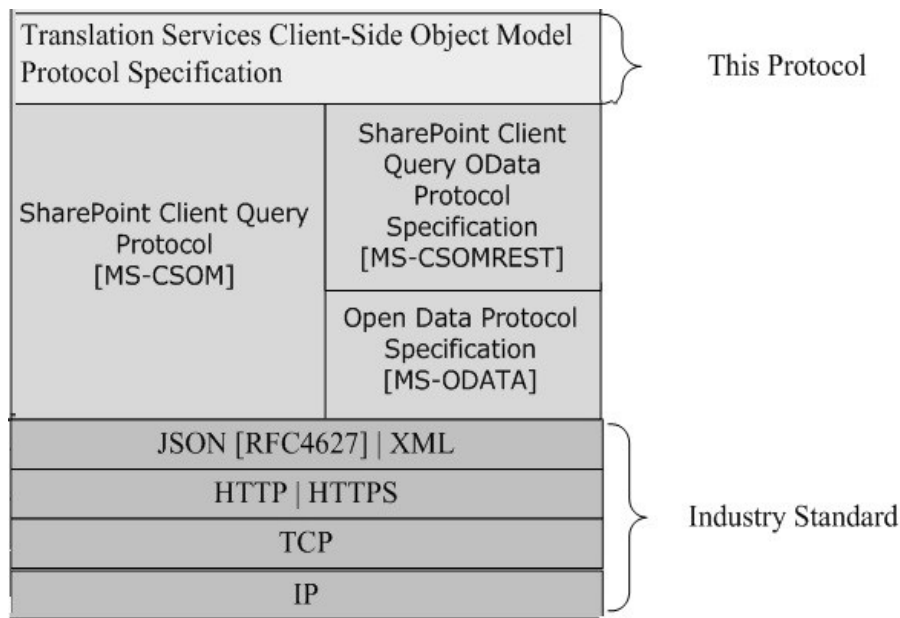
Figure 1: This protocol in relation to other protocols
