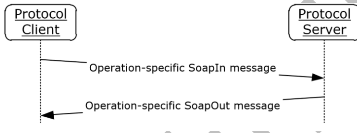
Figure 2: Message exchange between client and server
