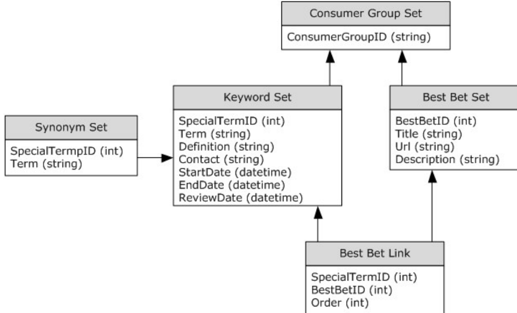
Figure 2: Best Bets and Keywords Abstract Data Model
