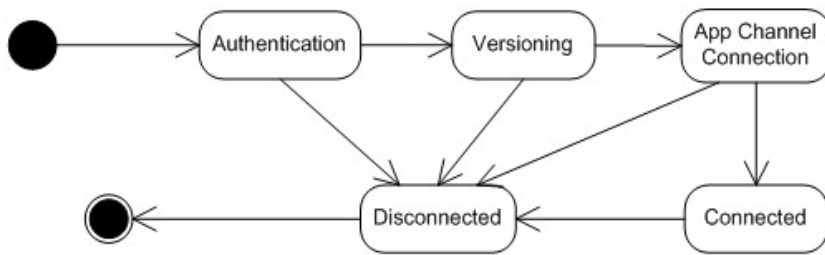
Figure 5: Client and server life-cycle stages
