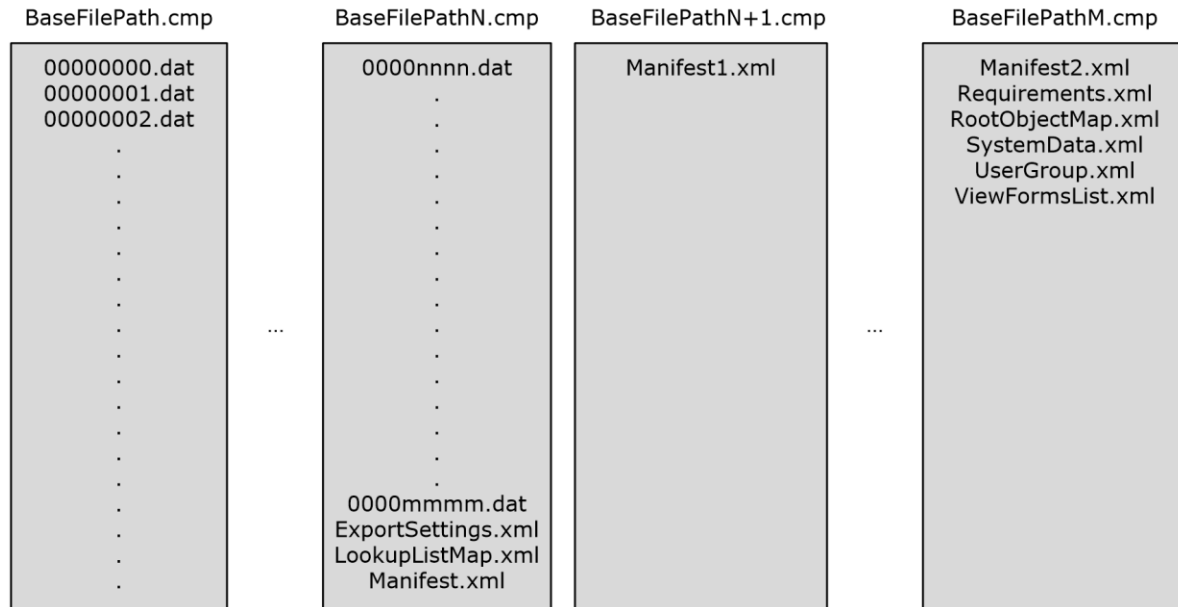
Figure 1: Deployment package chunking
