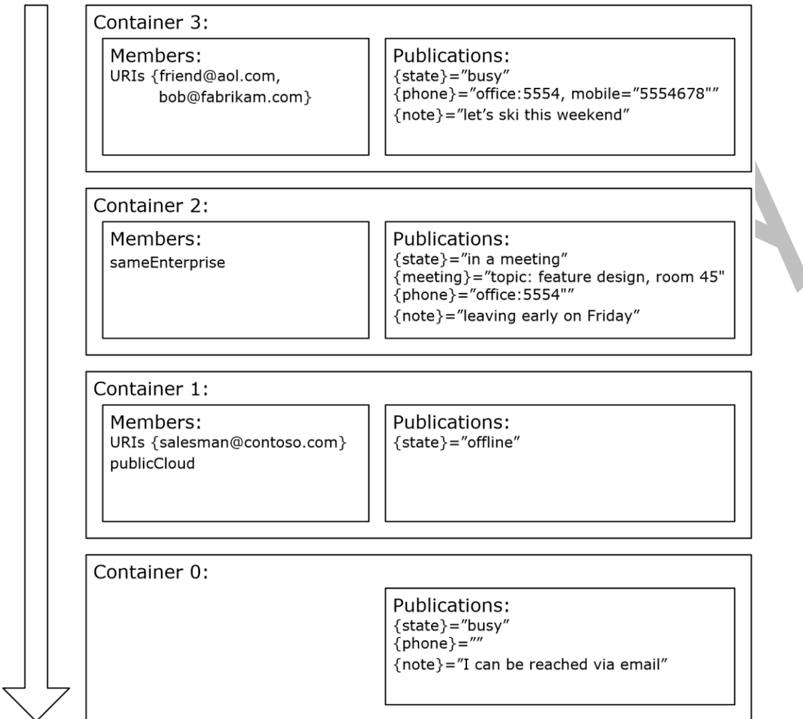
Figure 1: Container search order
