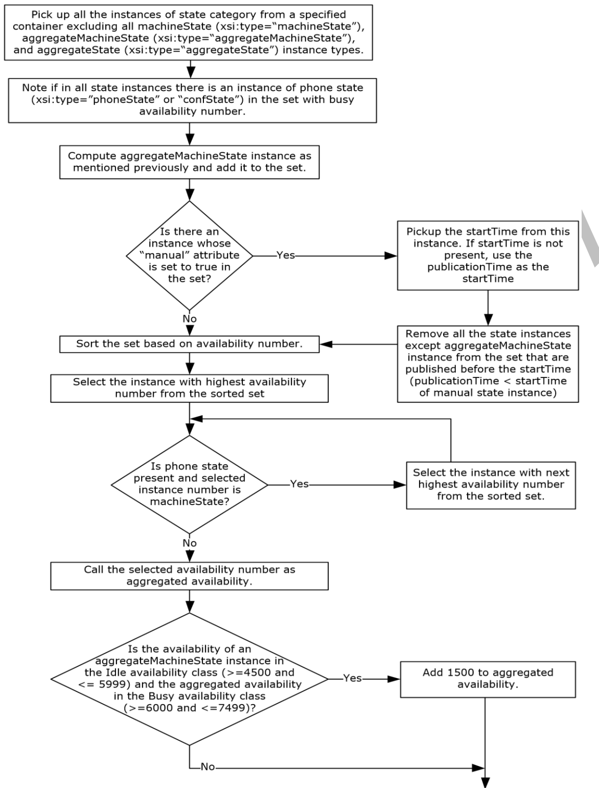
Figure 6: Computation of aggregated availability
