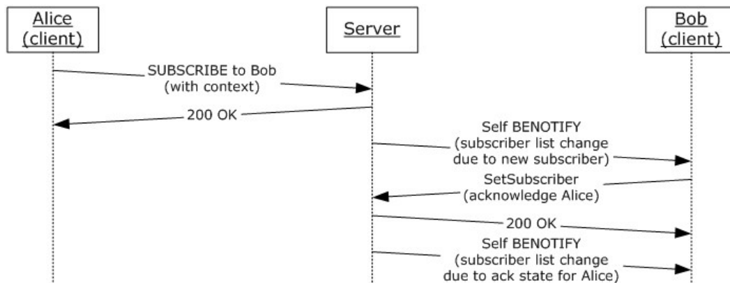
Figure 13: Sample call flow for setSubscriber
