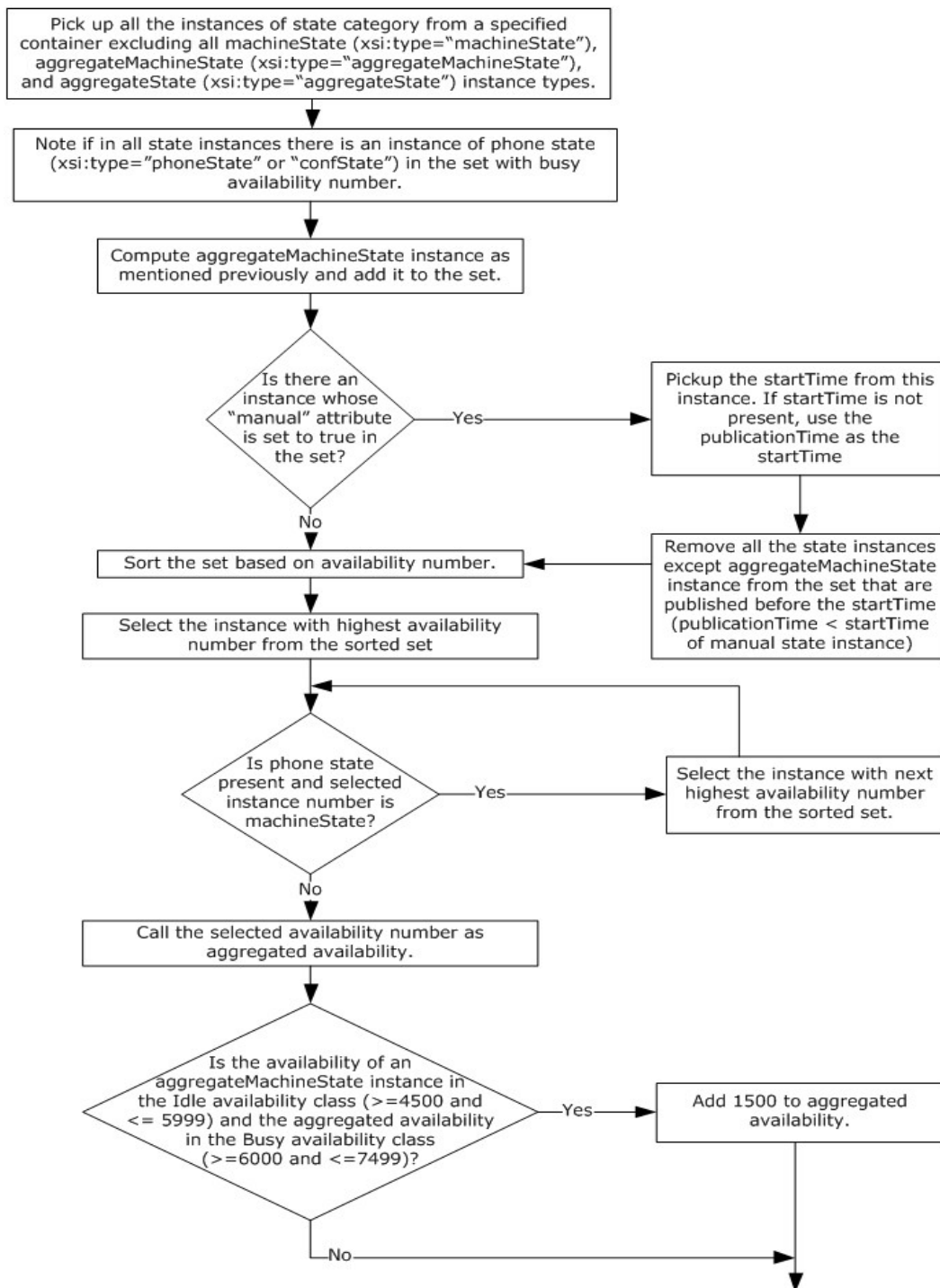
Figure 6: Computation of aggregated availability
