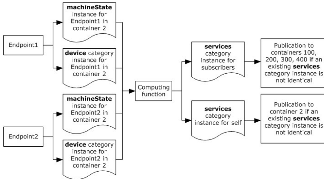
Figure 9: Aggregation of a device category
