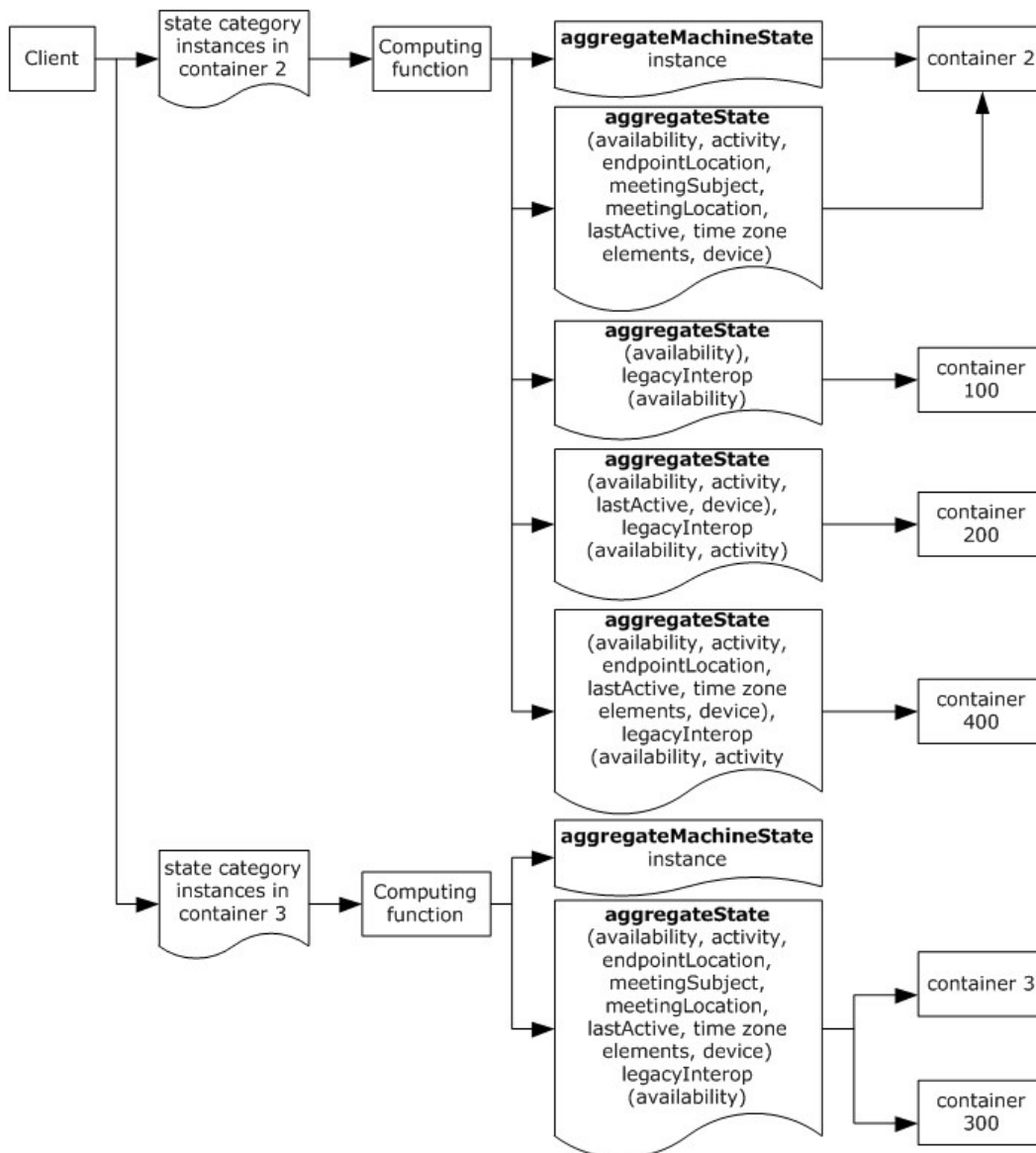
Figure 3: Aggregation of user's presence state
