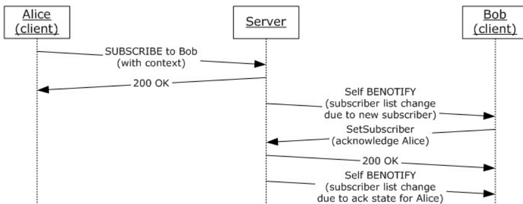
Figure 13: Sample call flow for setSubscriber
