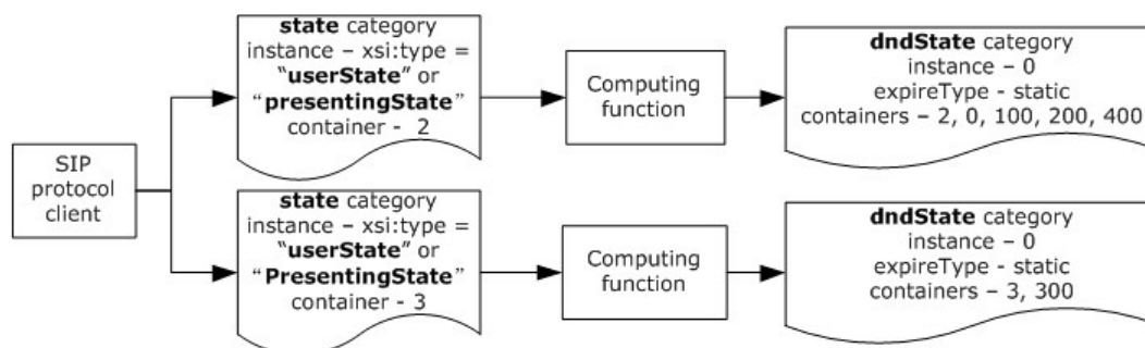
Figure 12: Creating a dndState category instance
