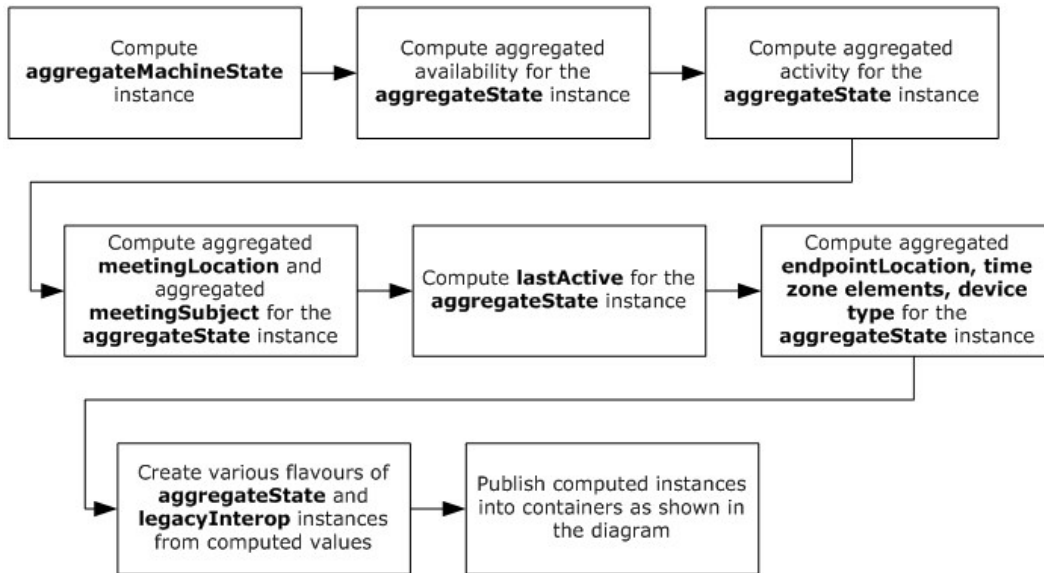
Figure 4: High-level call flow
