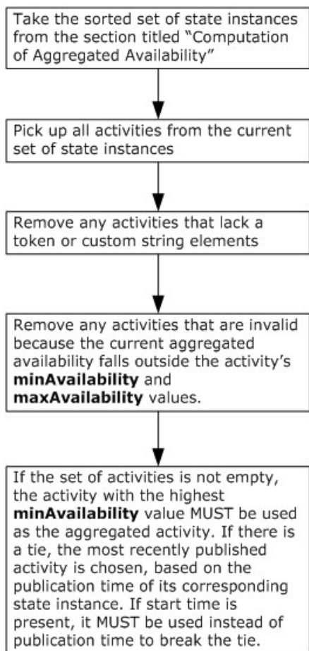
Figure 7: Computation of aggregated activity
