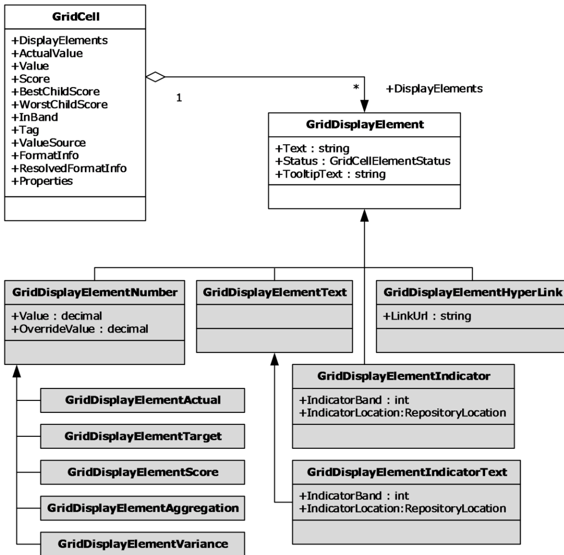
Figure 3: GridDisplayElement
