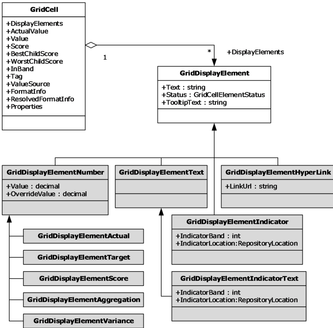
Figure 3: GridDisplayElement
