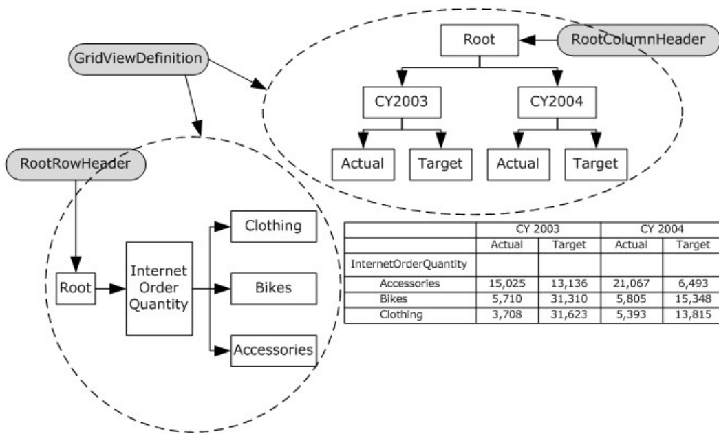
Figure 5: GridViewDefinition
