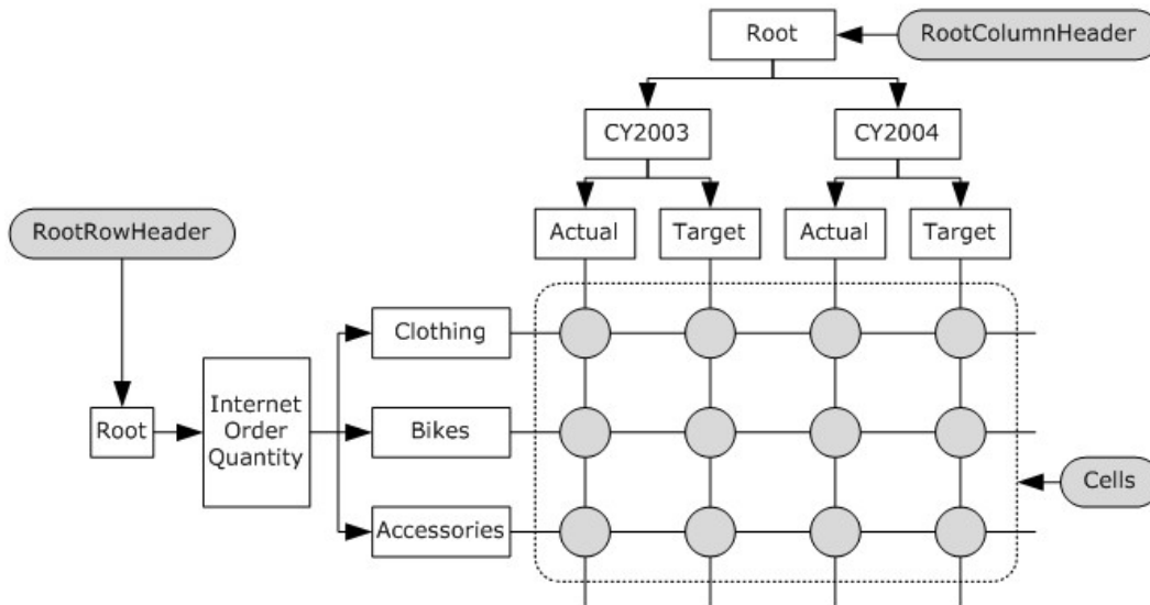
Figure 8: GridViewData
