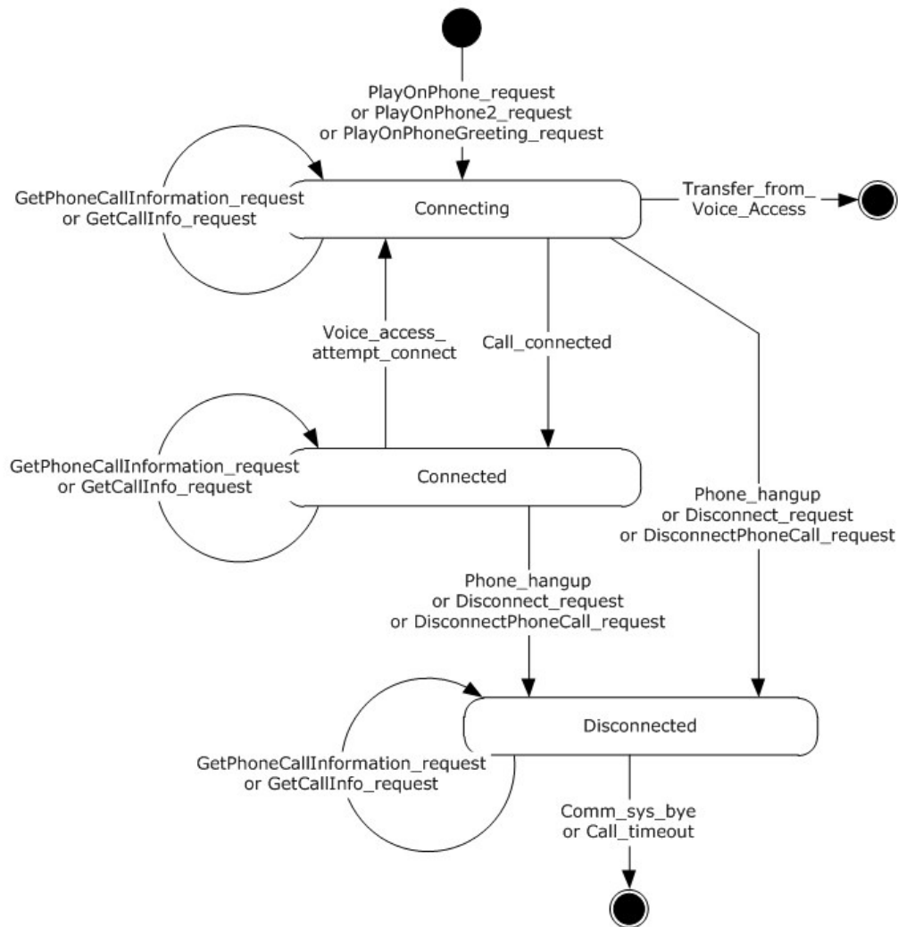
Figure 2: Phone Call Status subsystem abstract data model
