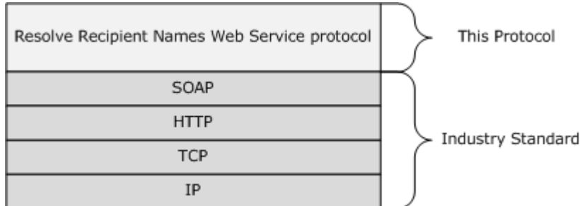
Figure 1: Resolve Recipient Names Web Service protocol HTTP stack
