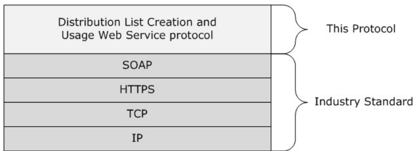
Figure 2: Distribution List Creation and Usage Web Service protocol HTTPS stack
