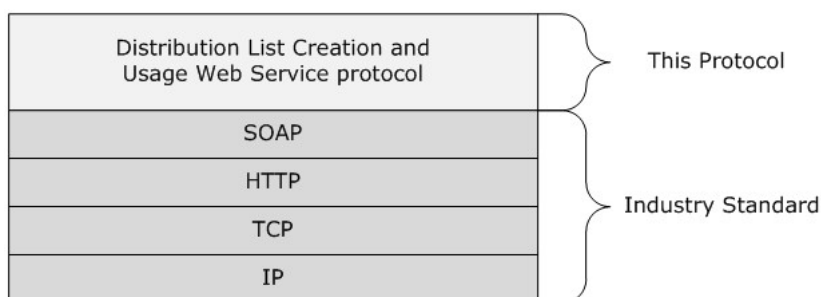
Figure 1: Distribution List Creation and Usage Web Service protocol HTTP stack
