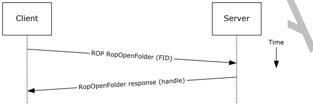
Figure 25: Opening a folder by using ROPs
