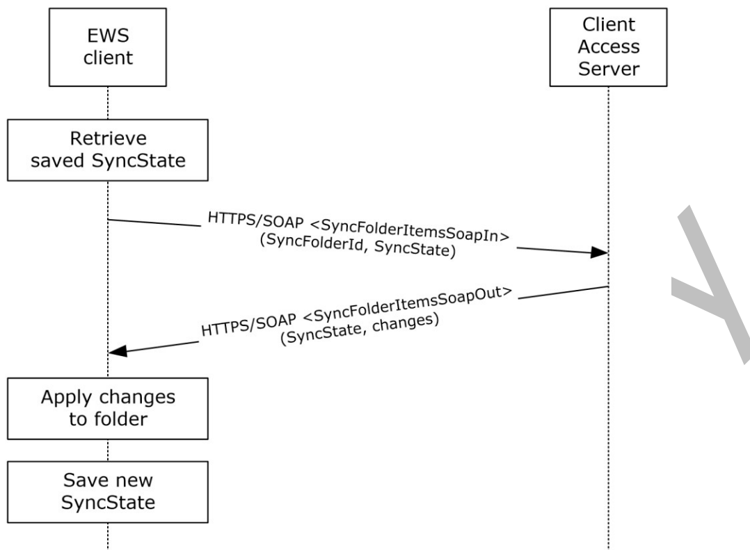
Figure 35: Synchronizing items by using Exchange Web Services
