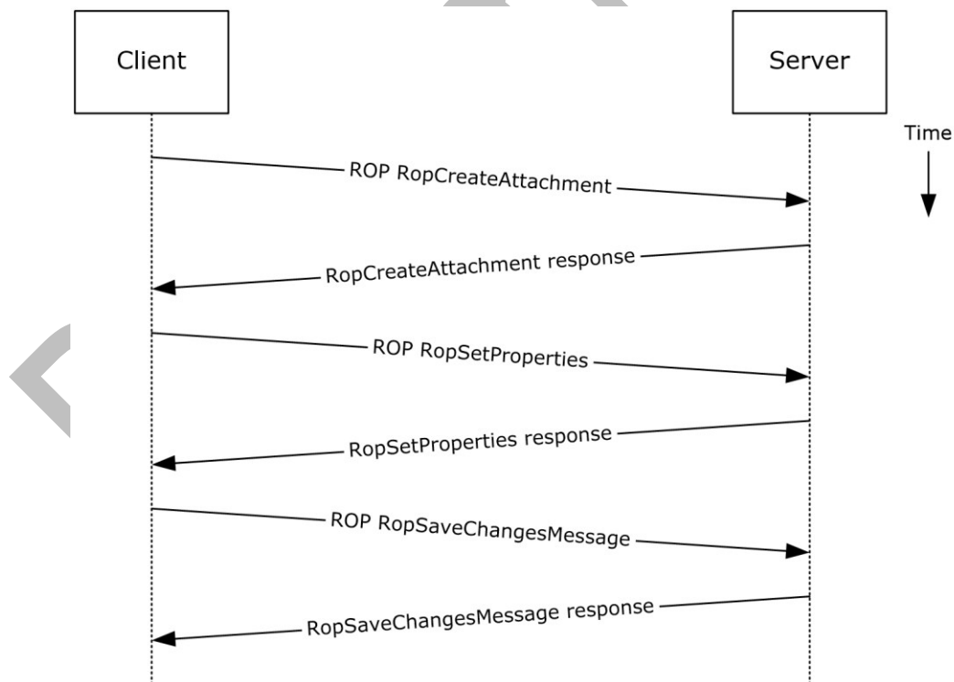
Figure 15: Adding an attachment by using ROPs
