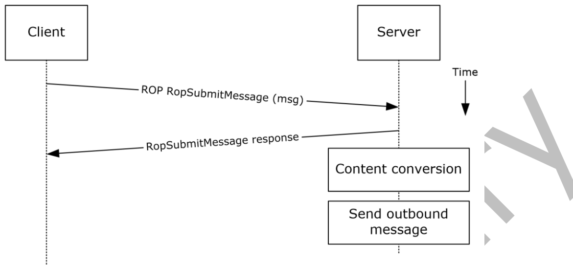
Figure 24: Sending a message to a remote recipient by using ROPs
