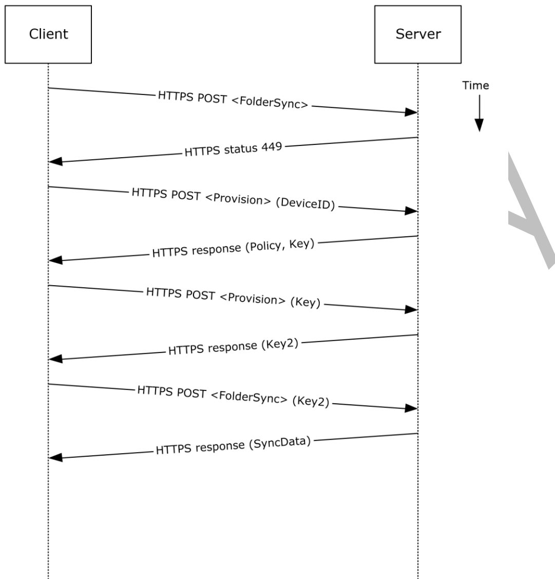
Figure 39: Provisioning a mobile client device by using Exchange ActiveSync
