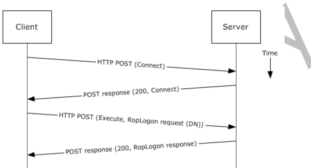
Figure 8: Logging on to a mailbox by using MAPI extensions for HTTP
