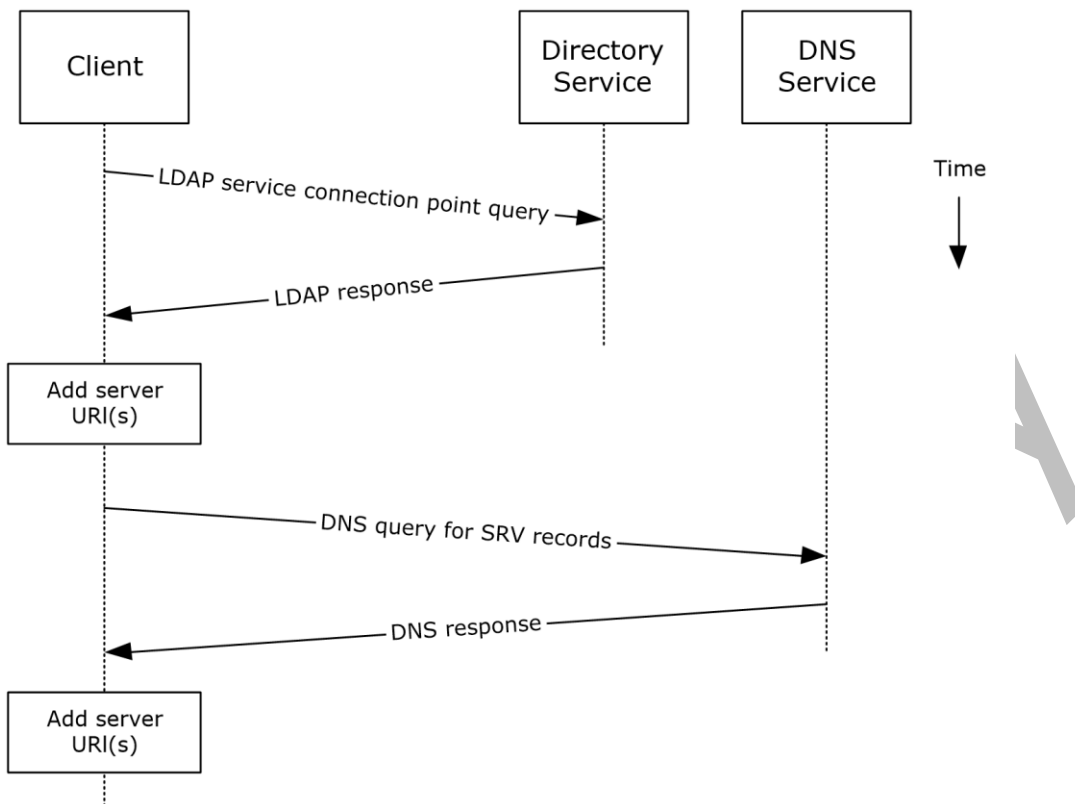
Figure 6: Server information discovery by using LDAP and DNS
