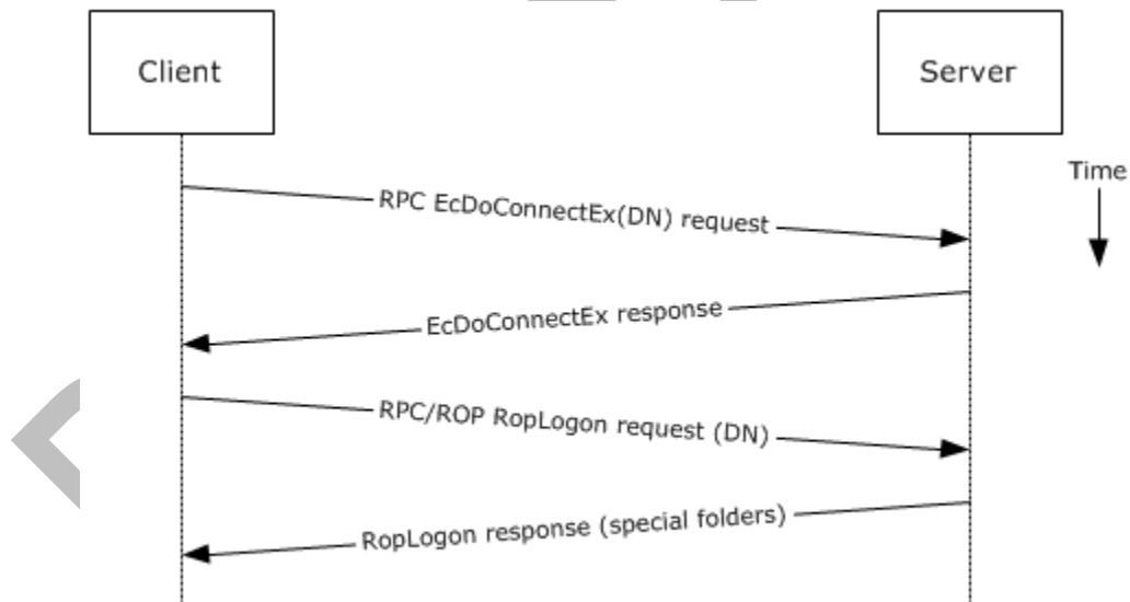
Figure 7: Logging on to a mailbox by using RPC
