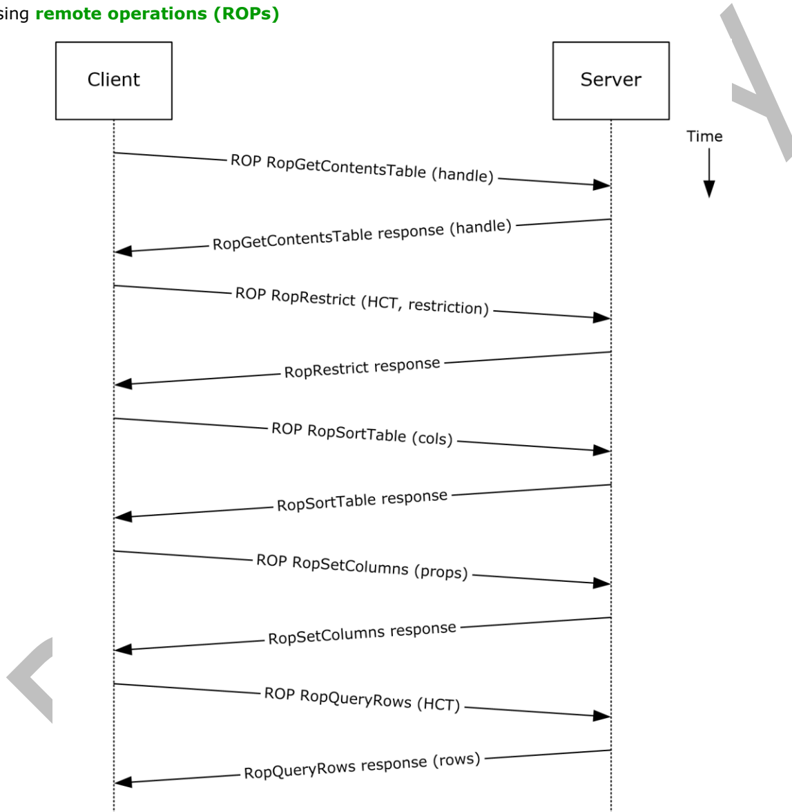
Figure 26: Finding folder items by using ROPs
