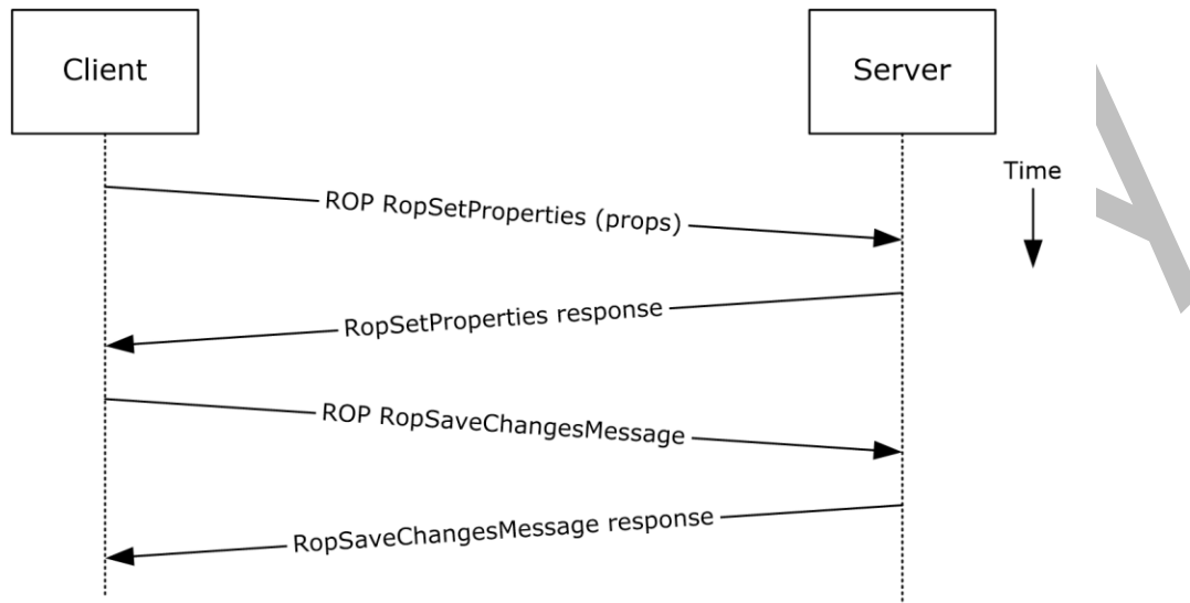
Figure 12: Creating a strongly typed message by using ROPs
