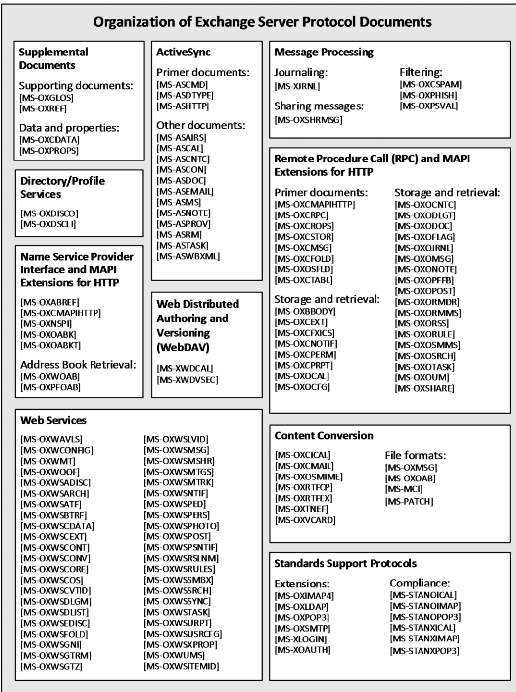
Figure 1: Organization of Microsoft Exchange protocol documents
