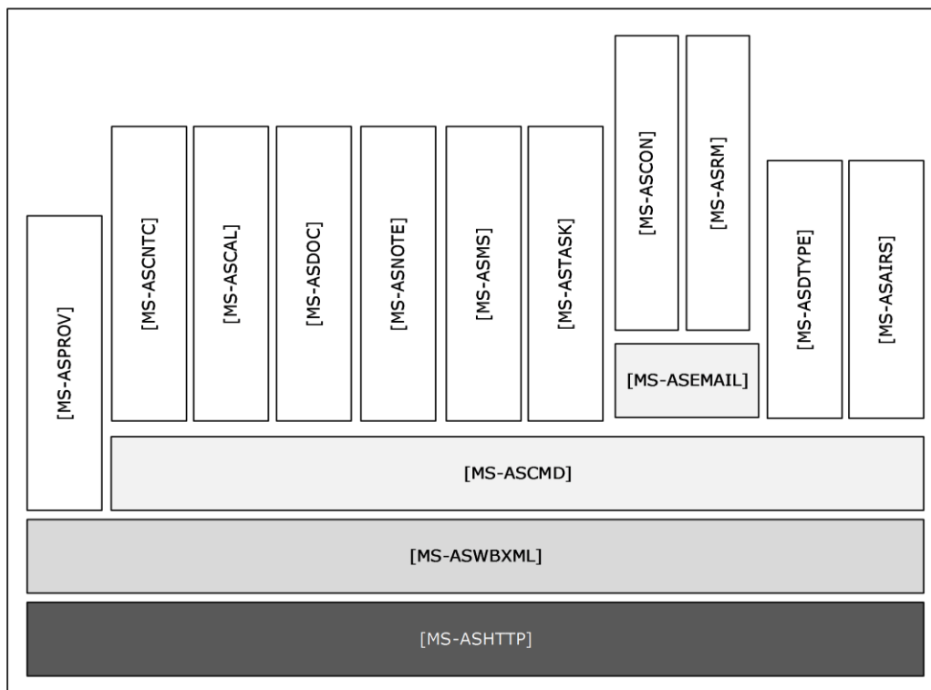
Figure 4: Exchange ActiveSync specifications
