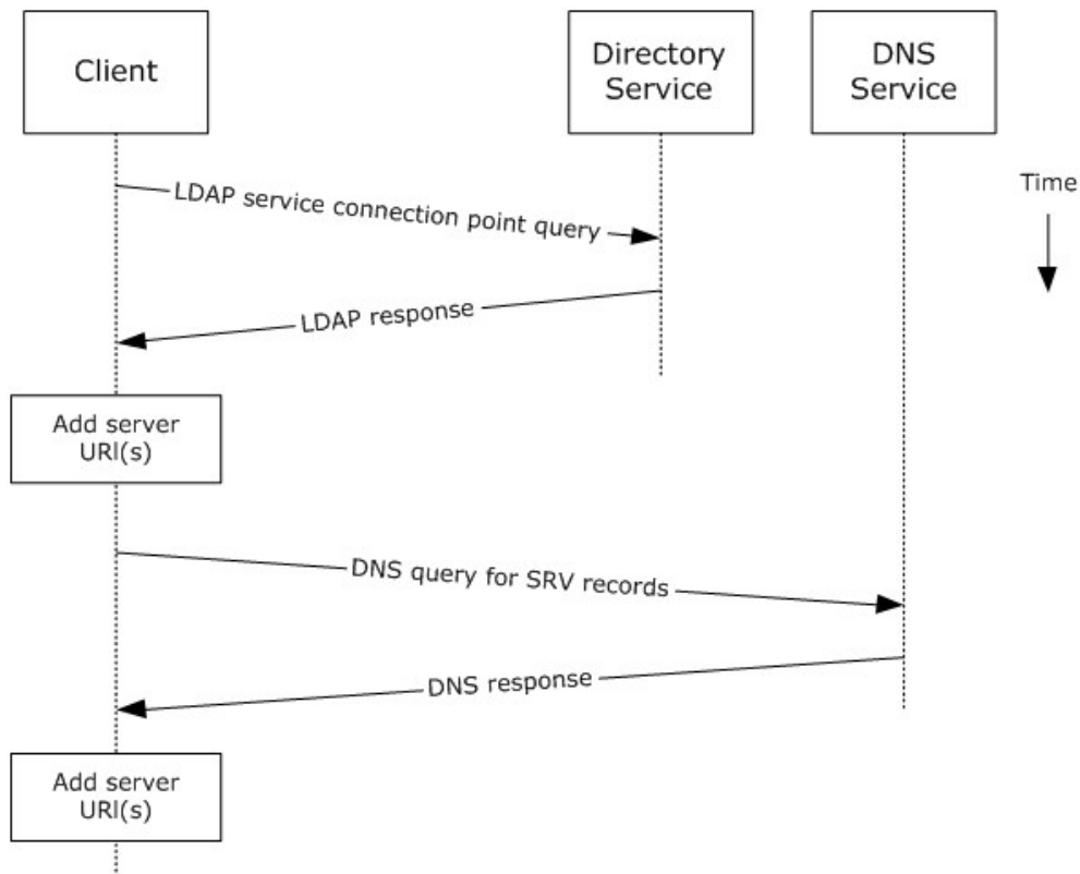
Figure 6: Server information discovery by using RPC
