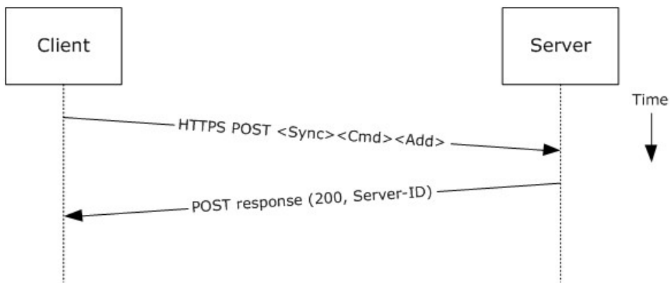
Figure 12: Creating a strongly typed message by using Exchange ActiveSync
