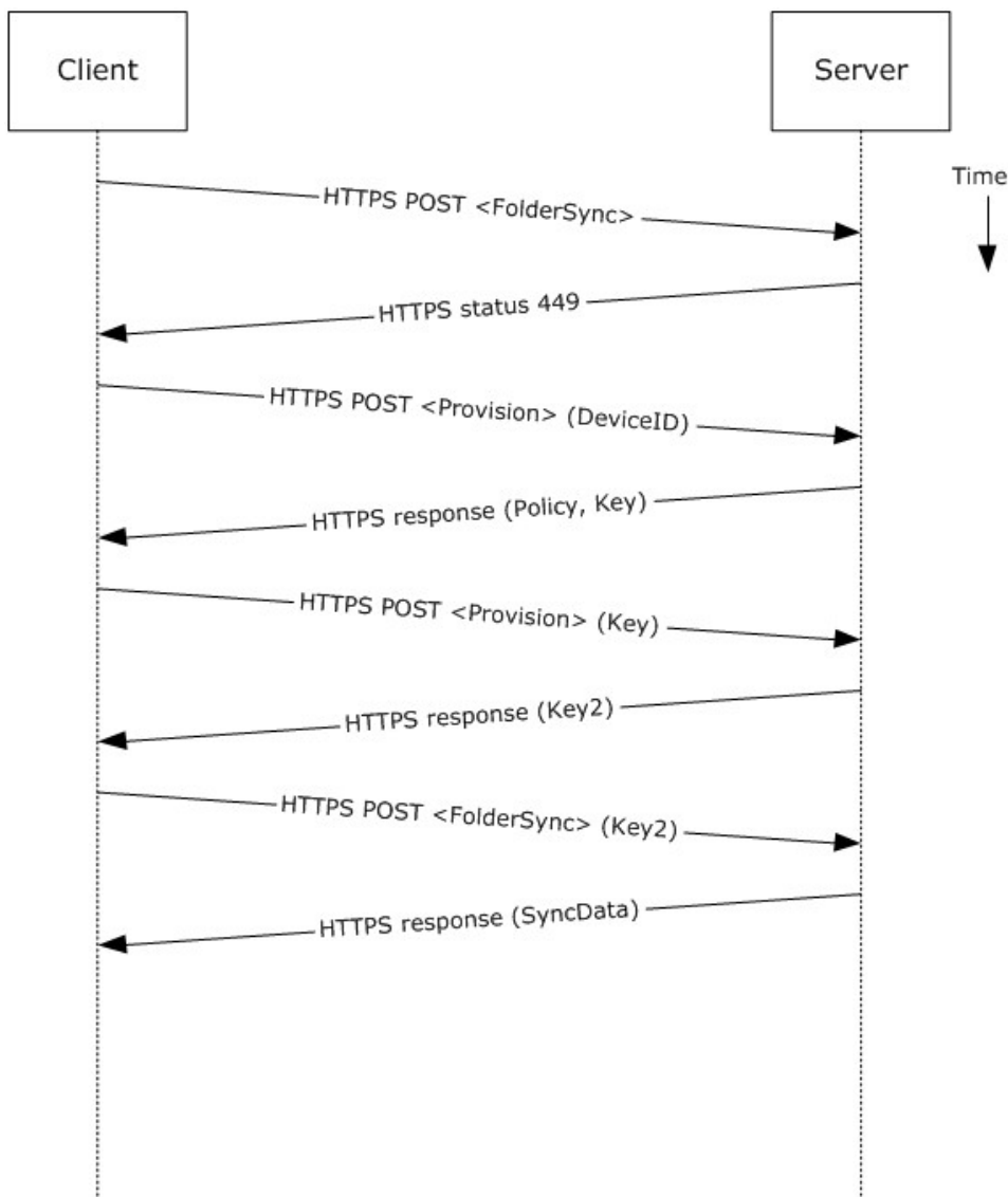
Figure 41: Provisioning a mobile client device by using Exchange ActiveSync
