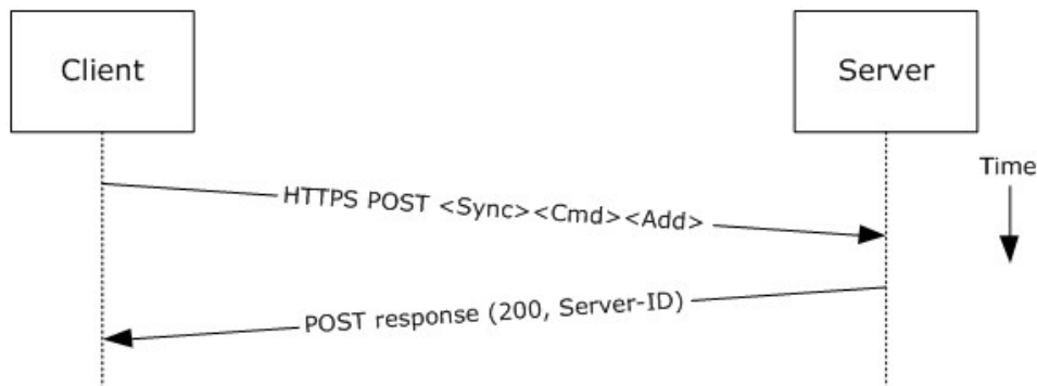
Figure 8: Creating a message by using Exchange ActiveSync
