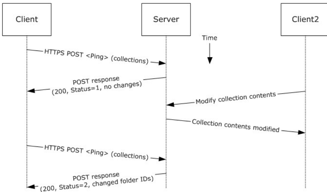
Figure 39: Registering for and receiving notifications by using Exchange ActiveSync
