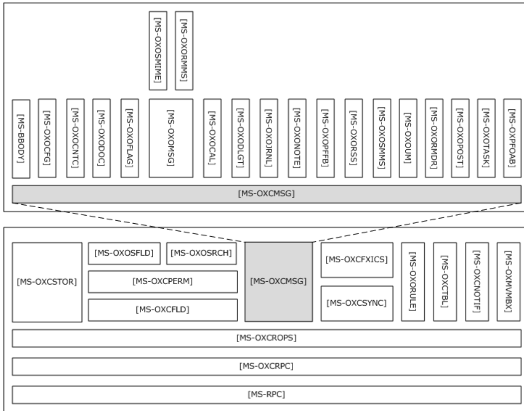
Figure 3: RPC primer/storage and retrieval protocol specifications
