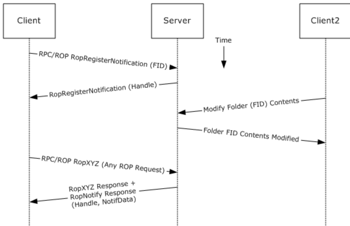
Figure 37: Registering for and receiving notifications using RPC
