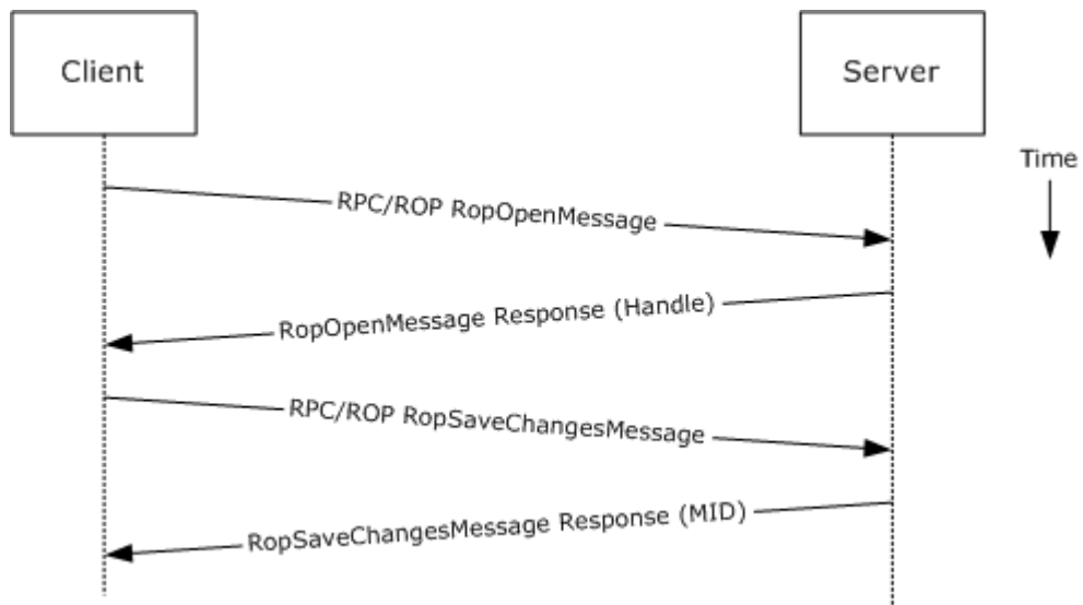
Figure 6: Creating a message using RPC
