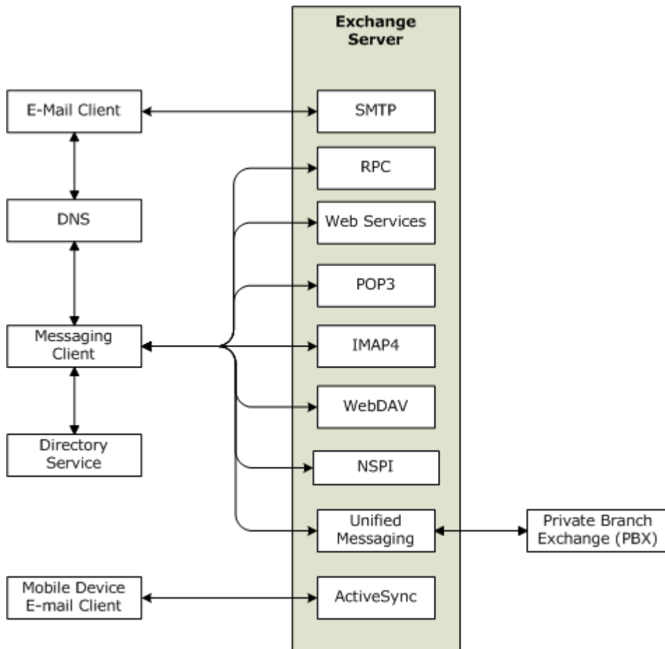
Figure 1: Functional architecture
