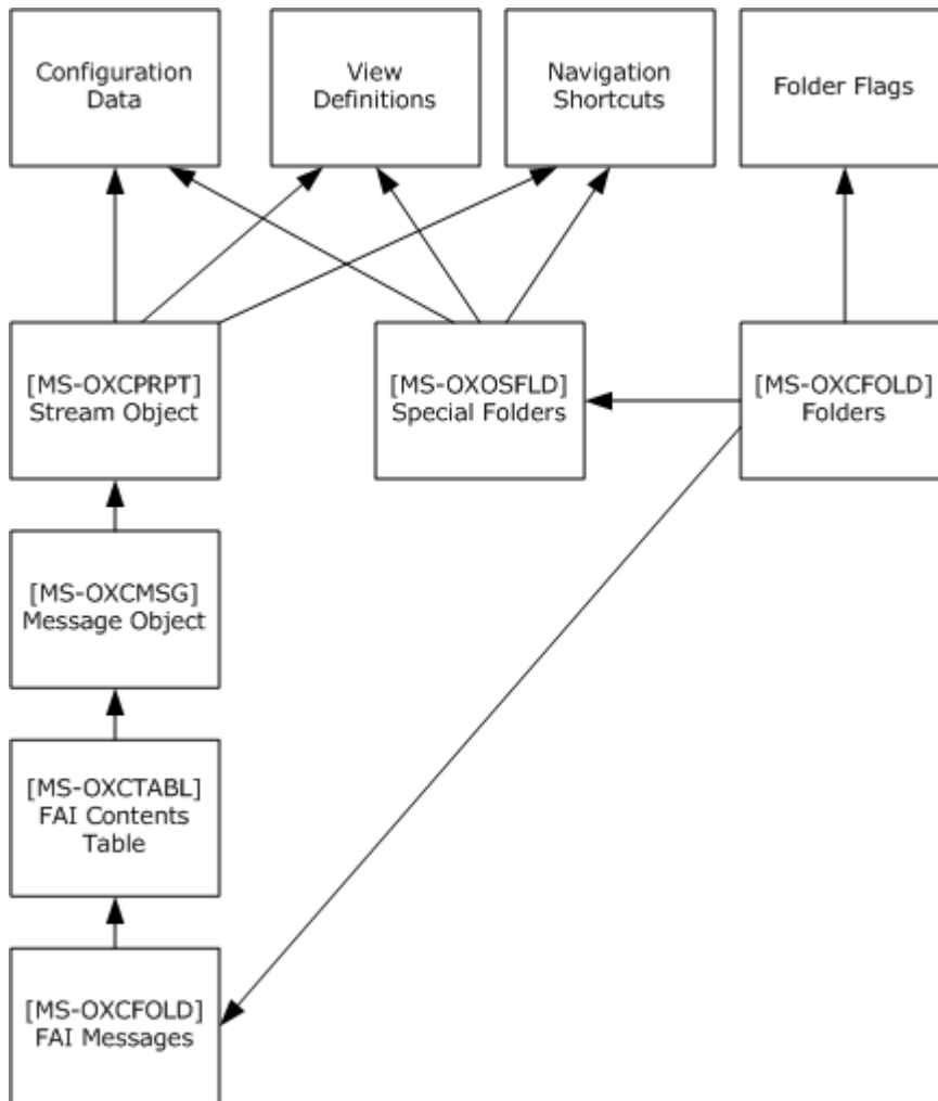
Figure 1: Protocol Stack
