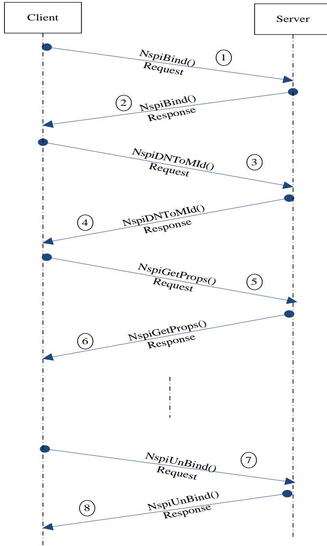
Figure 1: Call sequence
