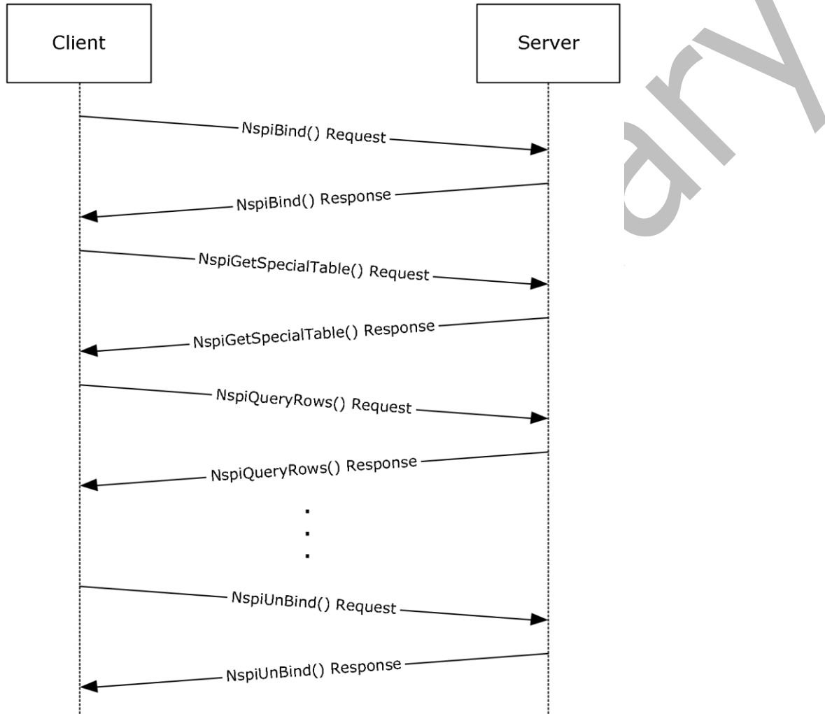
Figure 3: NSPI session message sequence example
