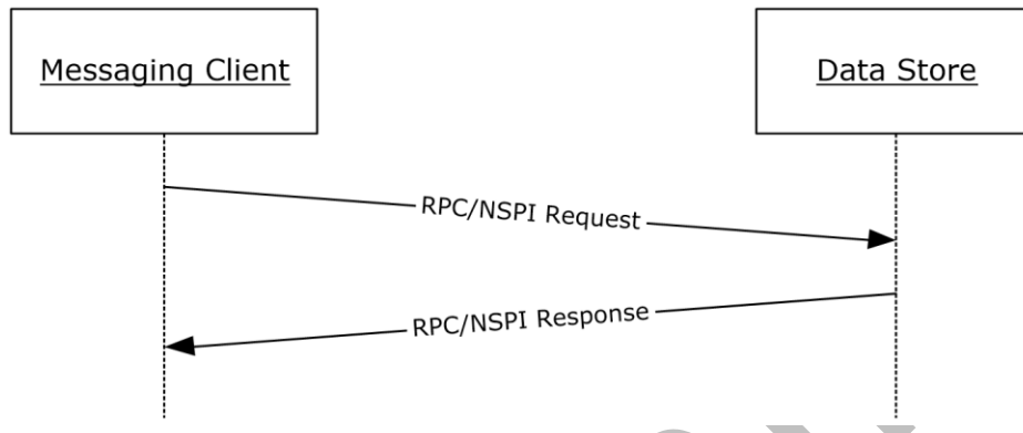
Figure 1: Exchange Server NSPI Protocol message sequence
