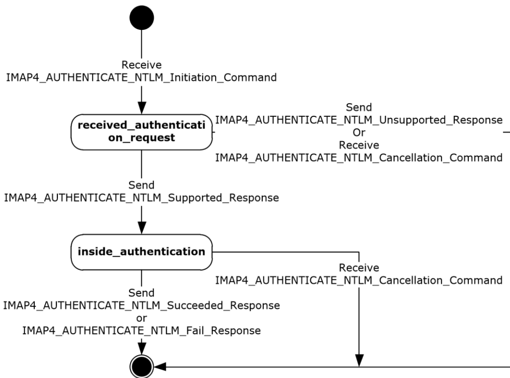
Figure 2: Server IMAP4 NTLM state model
