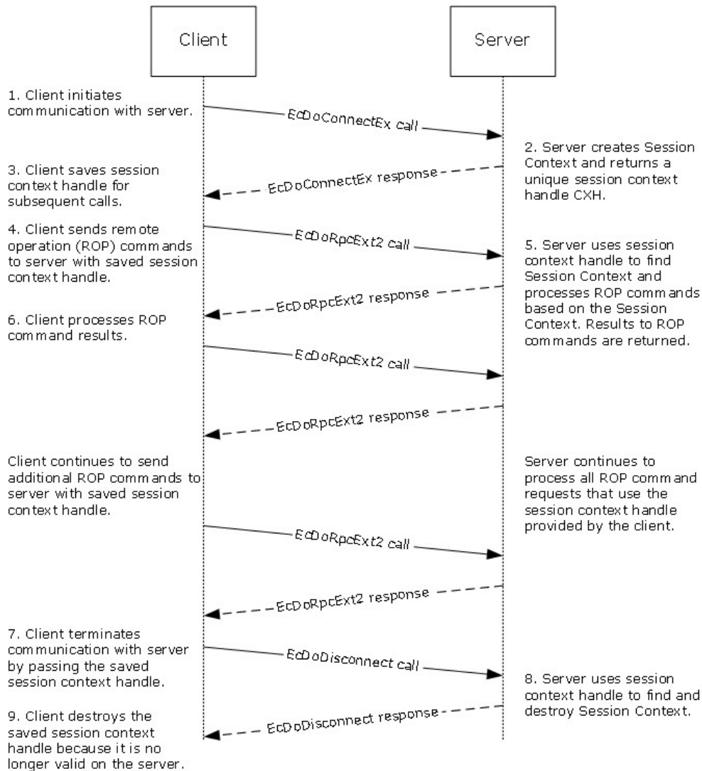
Figure 1: Client/server communications
