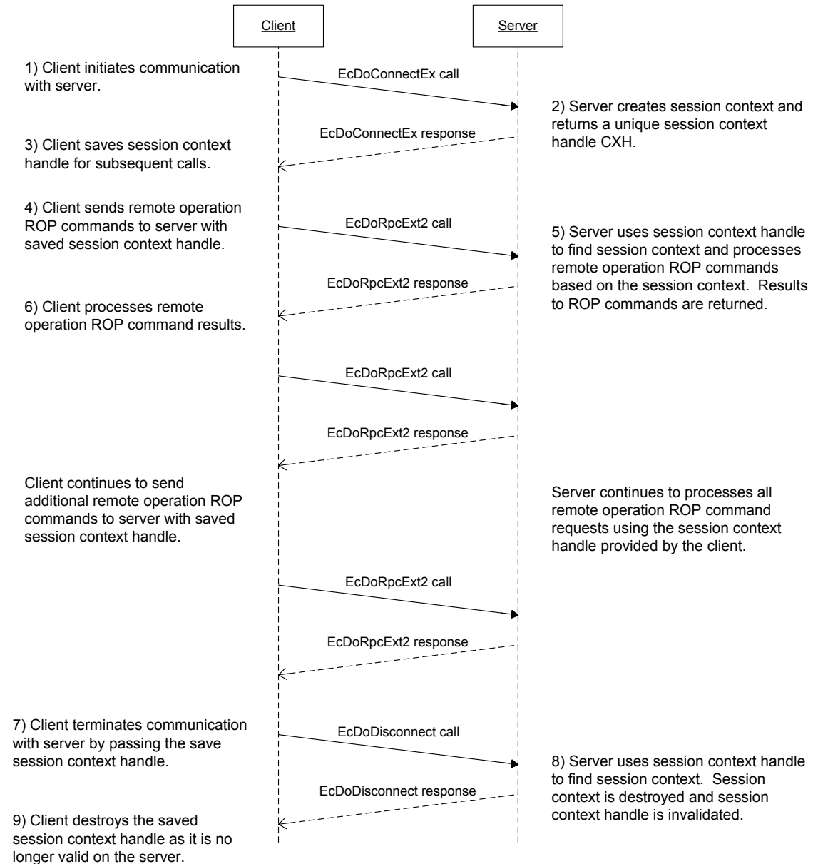
Figure 1: Client/server communications
