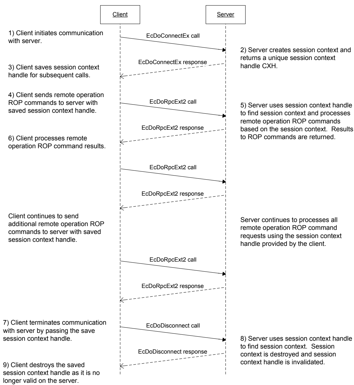
Figure 1: Client/server communications
