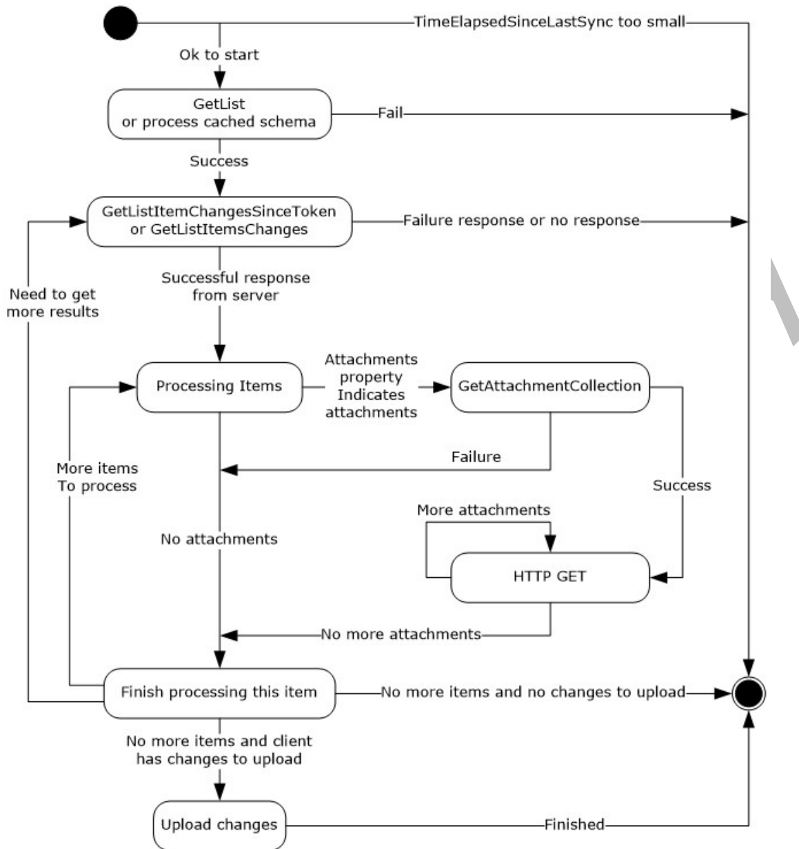
Figure 2: State diagram showing the sequence of decisions and operations performed by a protocol client
