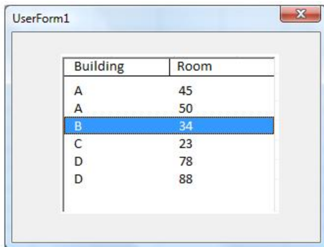
Figure 5: ListBox control
