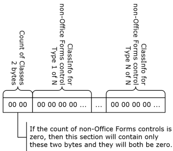
Figure 20: ClassTable structure
