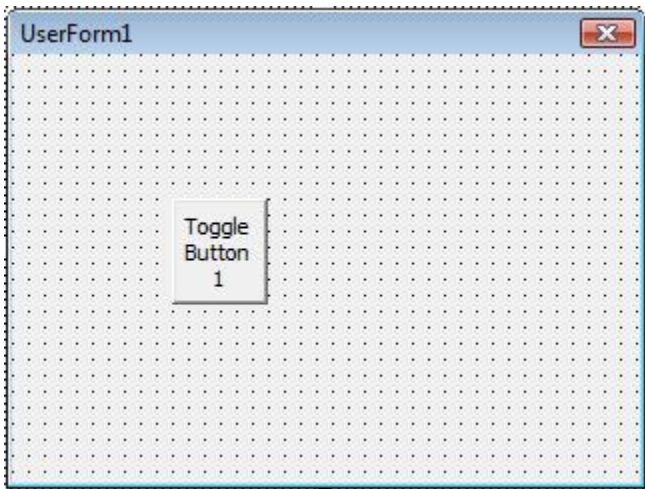
Figure 8: ToggleButton control
