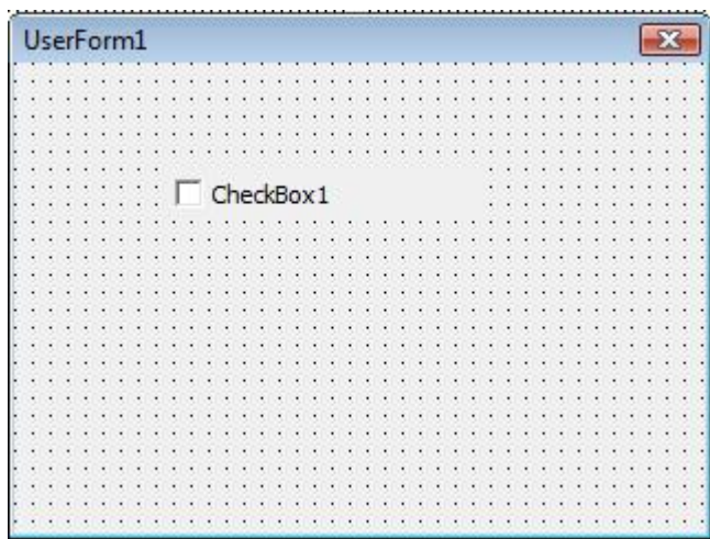
Figure 3: CheckBox control
