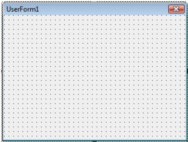
Figure 1: UserForm control
