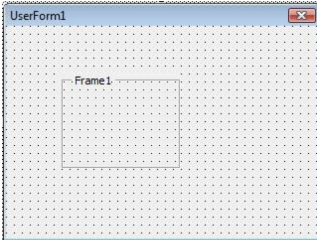
Figure 2: Frame control
