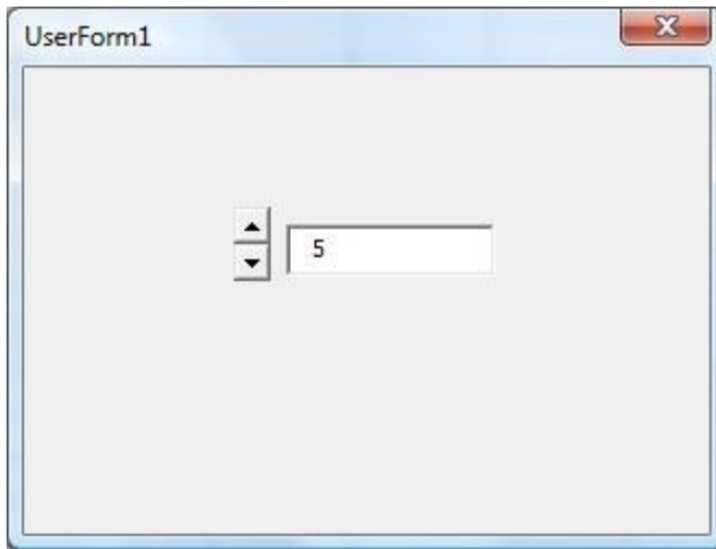
Figure 15: SpinButton control
