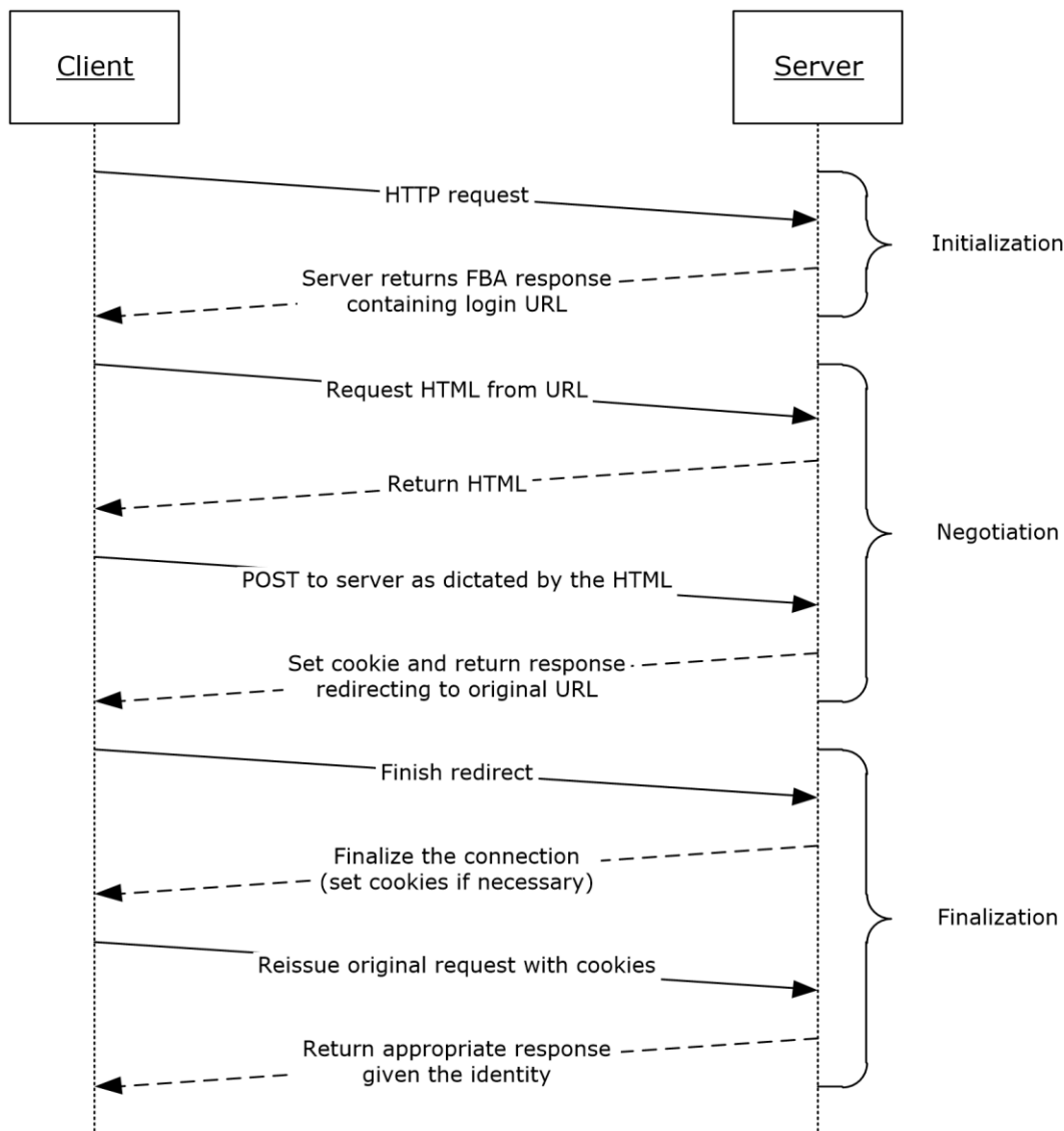
Figure 1: Sequence diagram
