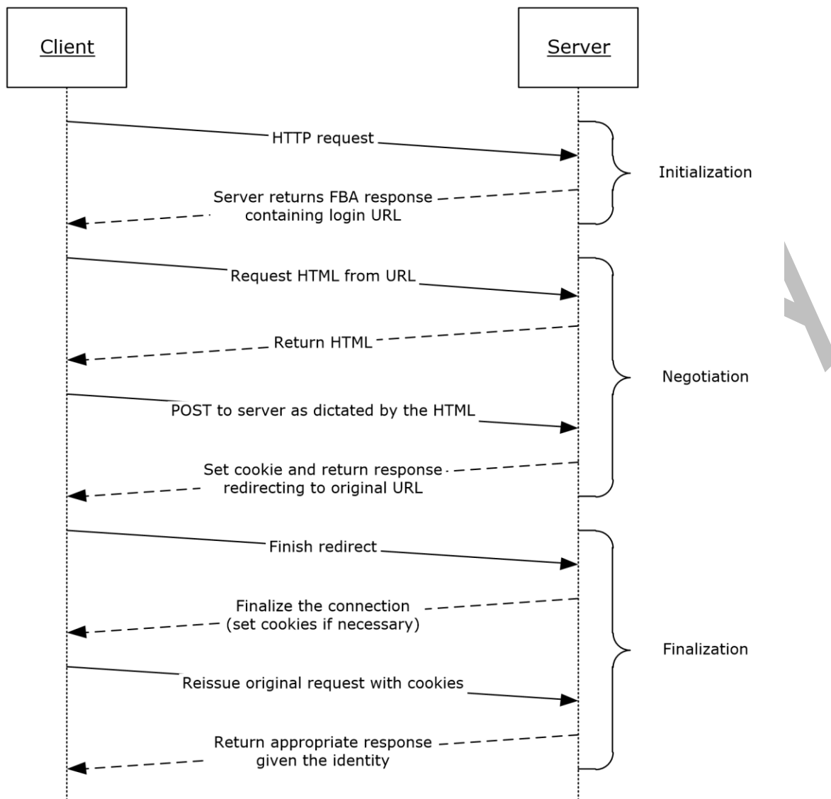
Figure 1: Sequence diagram
