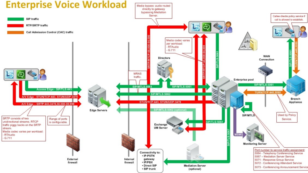
Figure 4: Enterprise voice workload
