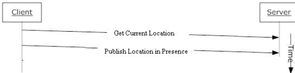
Figure 35: Process for getting location and changing presence.
