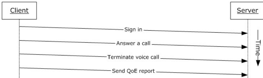
Figure 30: Sequence for accepting an inbound call to Office Communicator
