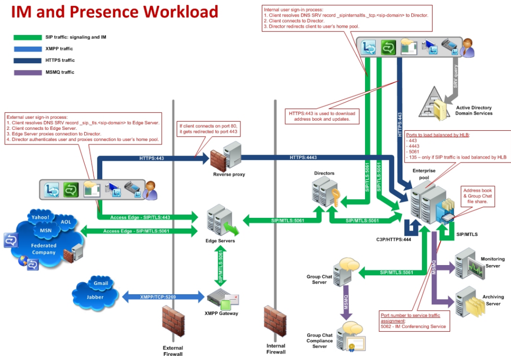
Figure 2: IM and presence workload
