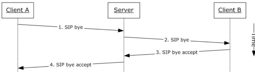
Figure 19: Steps for terminating a voice call
