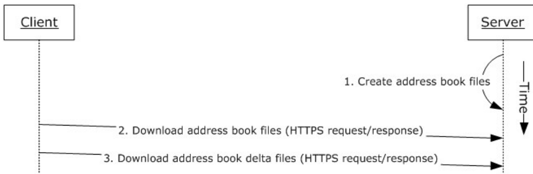
Figure 11: Steps for downloading the address book
