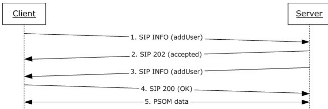
Figure 24: Steps for sharing a whiteboard
