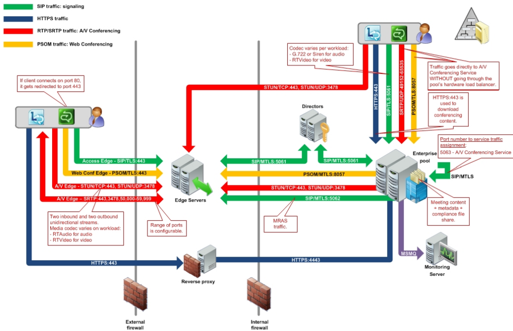
Figure 5: A/V and Web Conferencing Workload
