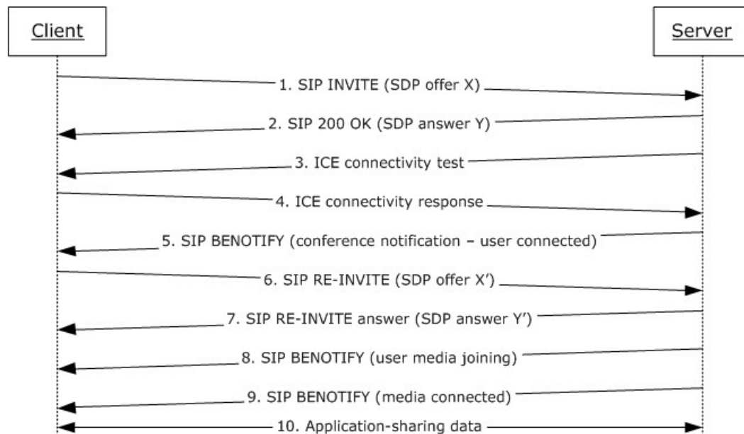
Figure 23: Steps for sharing a desktop
