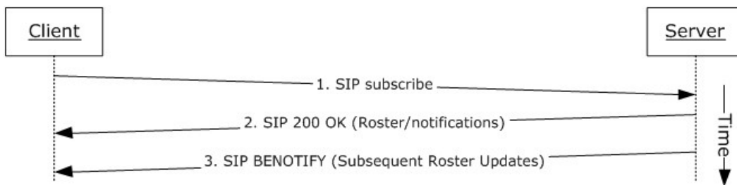
Figure 22: Steps for subscribing to conference events
