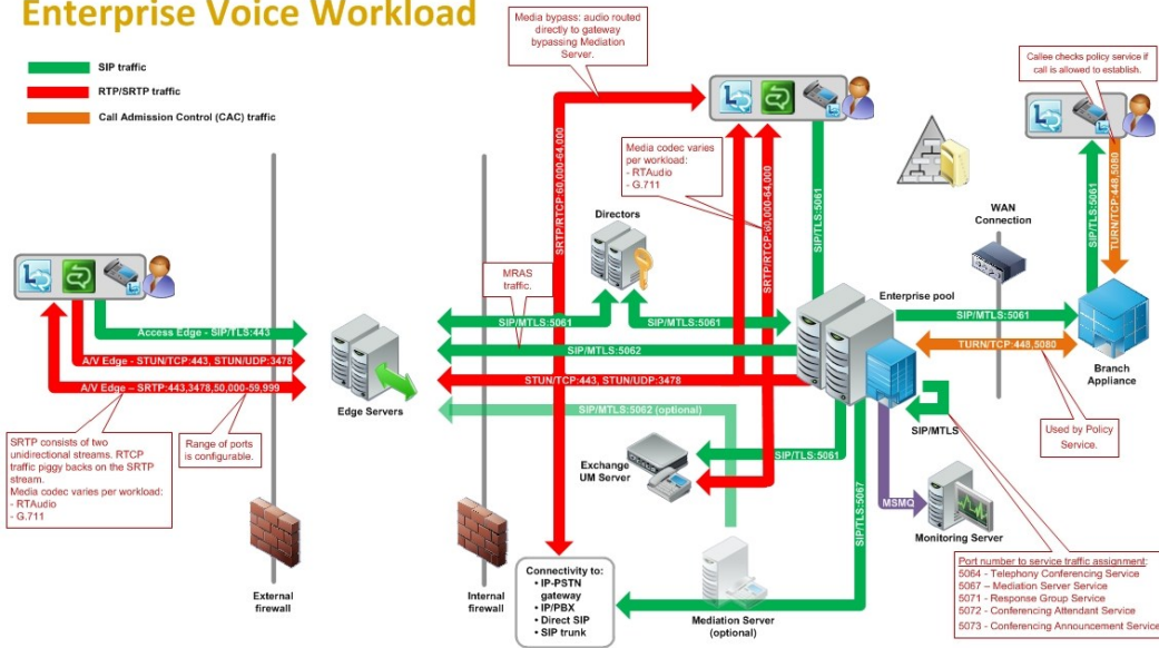
Figure 4: Enterprise voice workload
