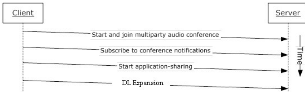
Figure 34: Sequence for starting a conference, joining with multiparty audio, and starting application-sharing, Distribution List (DL) Expansion
