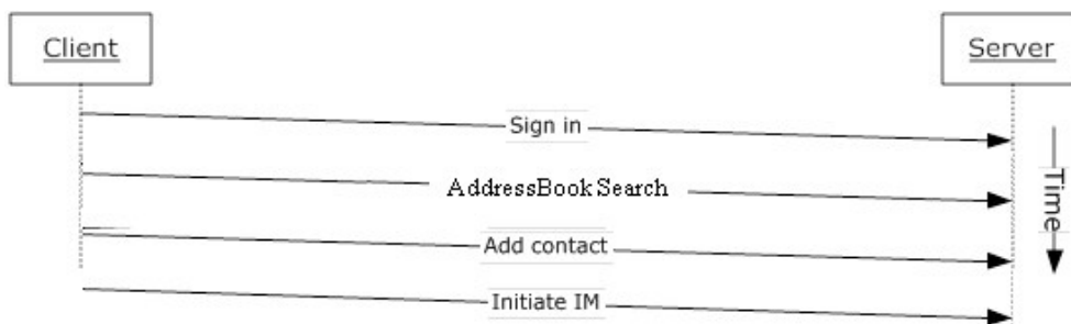
Figure 26: Sequence for sending an instant message to a contact
