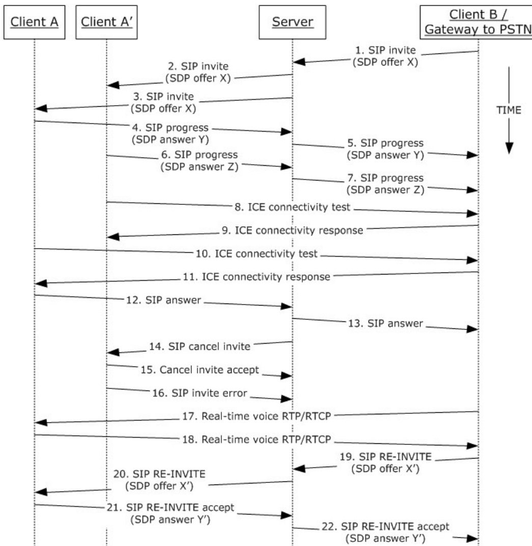
Figure 18: Steps for accepting a voice call
