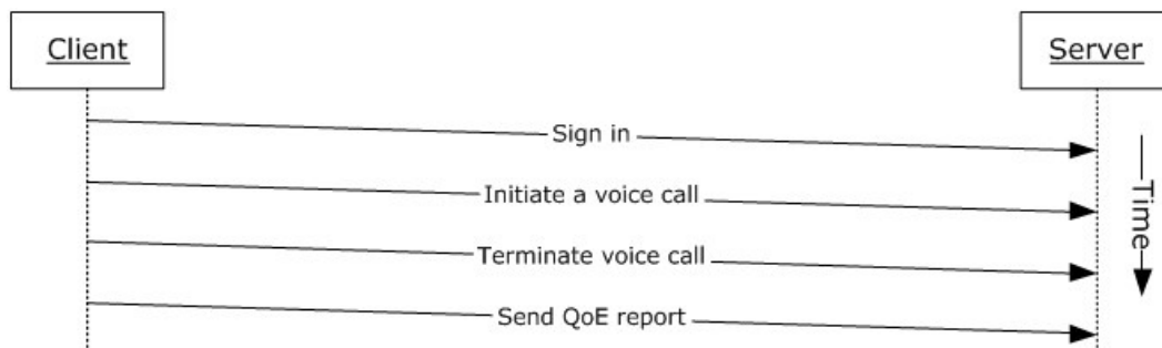
Figure 28: Sequence for making a call from Office Communicator
