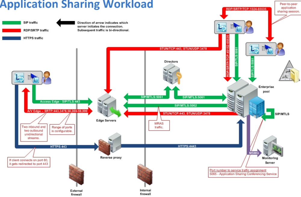
Figure 3: Application sharing workload
