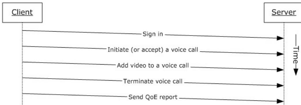
Figure 32: Sequence for adding video to a voice call from Office Communicator
