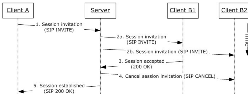
Figure 15: Steps for using multiple endpoints (5)
