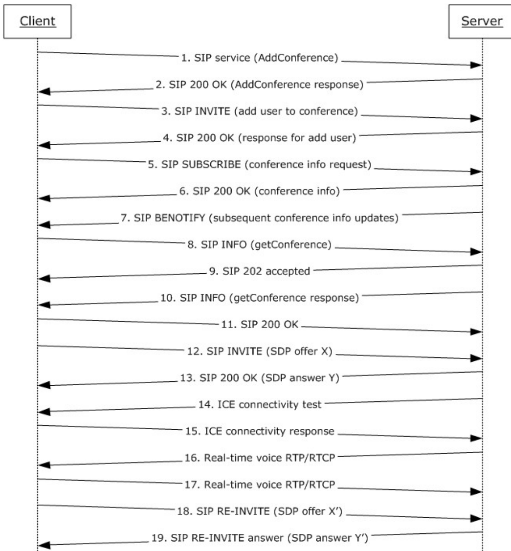
Figure 16: Steps for starting and joining a multiparty audio conference
