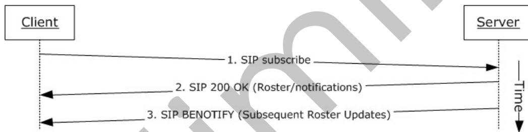
Figure 18: Steps for subscribing to conference events
