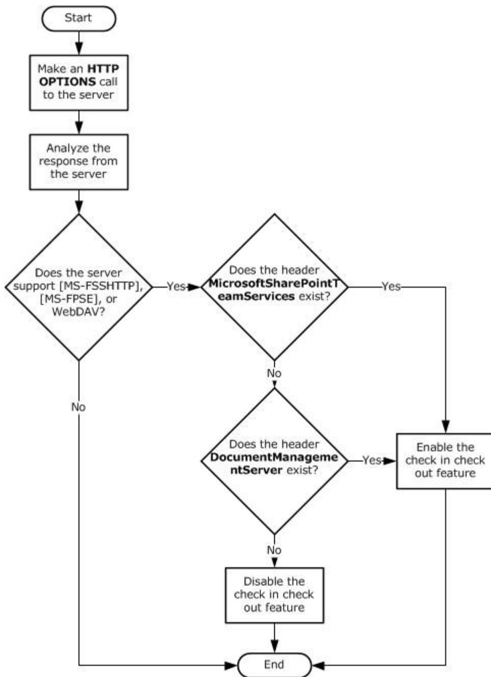
Figure 17: Process for enabling the check in and check out features in client applications
