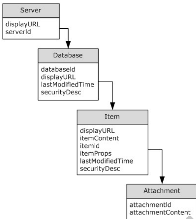
Figure 2: Object Hierarchy
